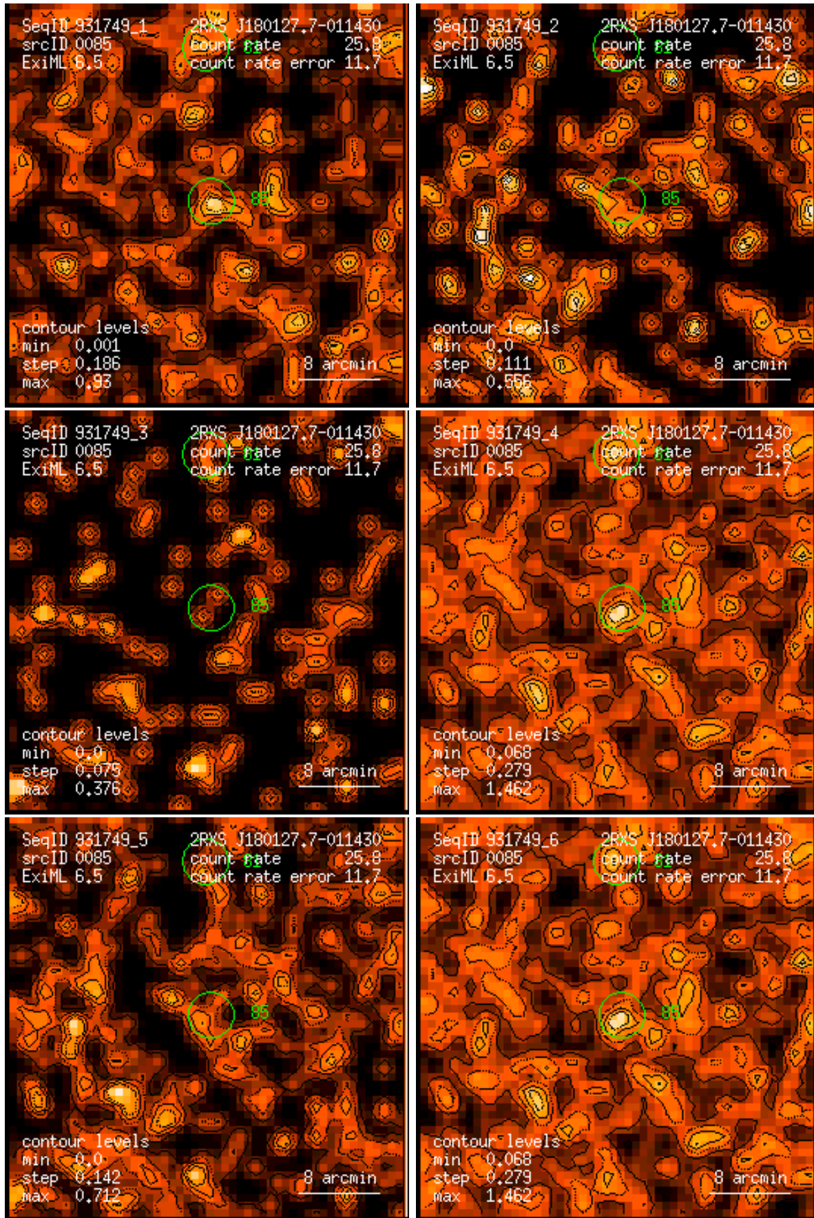
Figure 85: RASS 931749: detection 0085: band rate images, Gaussian filter: (1) PSPC channels 11 – 41, (2) 52 – 90, (3) 91 – 201, (4) 11 – 235, (5) 52 – 201, (6) 11 – 201. Broad band rates in counts/ks. Band rate contour levels in counts/ks/arcmin 2 .
