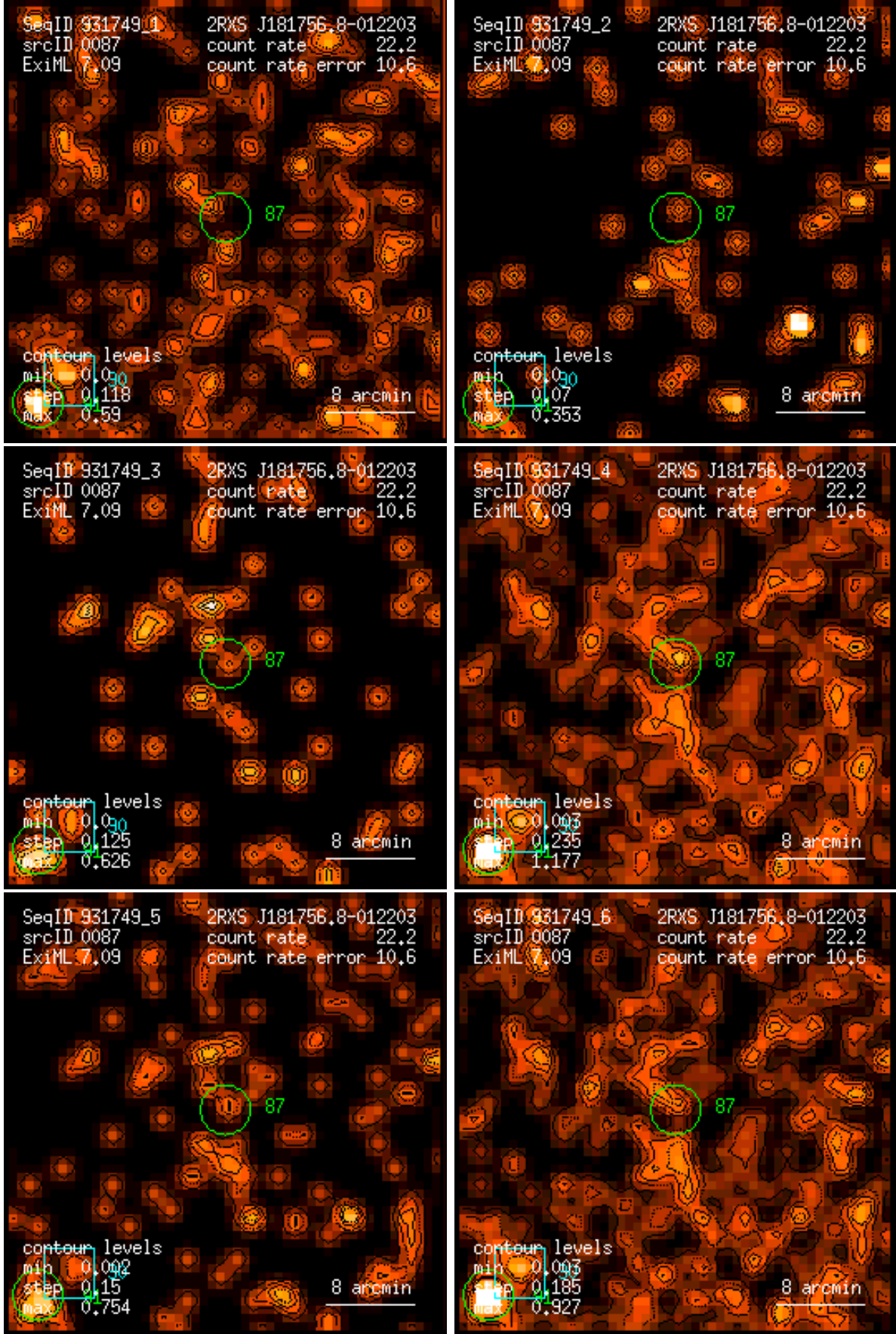
Figure 87: RASS 931749: detection 0087: band rate images, Gaussian filter: (1) PSPC channels 11 – 41, (2) 52 – 90, (3) 91 – 201, (4) 11 – 235, (5) 52 – 201, (6) 11 – 201. Broad band rates in counts/ks. Band rate contour levels in counts/ks/arcmin 2 .
