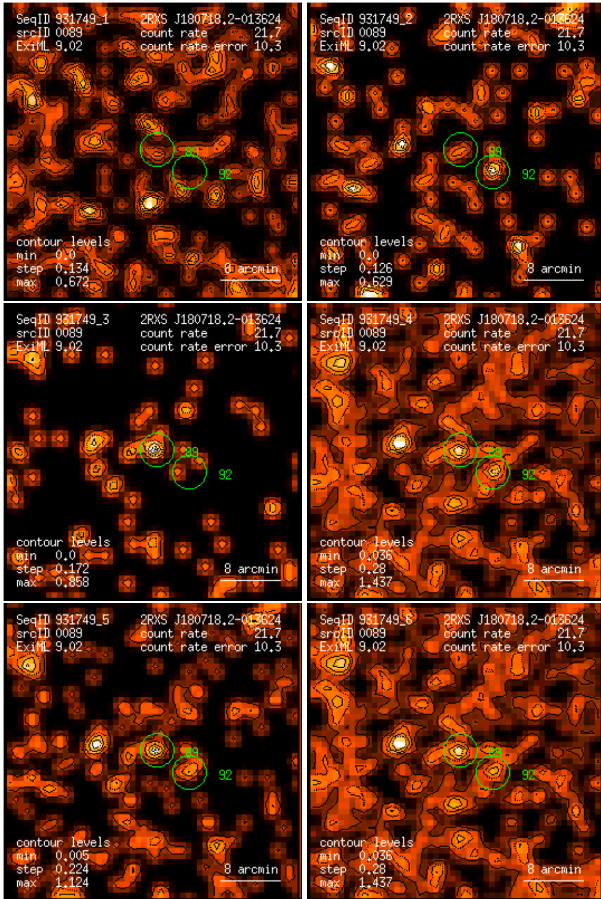
Figure 89: RASS 931749: detection 0089: band rate images, Gaussian filter: (1) PSPC channels 11 – 41, (2) 52 – 90, (3) 91 – 201, (4) 11 – 235, (5) 52 – 201, (6) 11 – 201. Broad band rates in counts/ks. Band rate contour levels in counts/ks/arcmin 2 .
