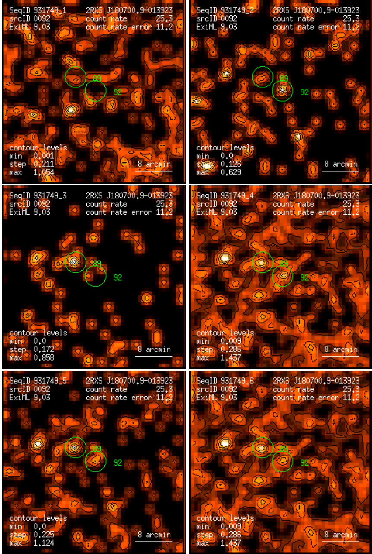
Figure 92: RASS 931749: detection 0092: band rate images, Gaussian filter: (1) PSPC channels 11 – 41, (2) 52 – 90, (3) 91 – 201, (4) 11 – 235, (5) 52 – 201, (6) 11 – 201. Broad band rates in counts/ks. Band rate contour levels in counts/ks/arcmin 2 .
