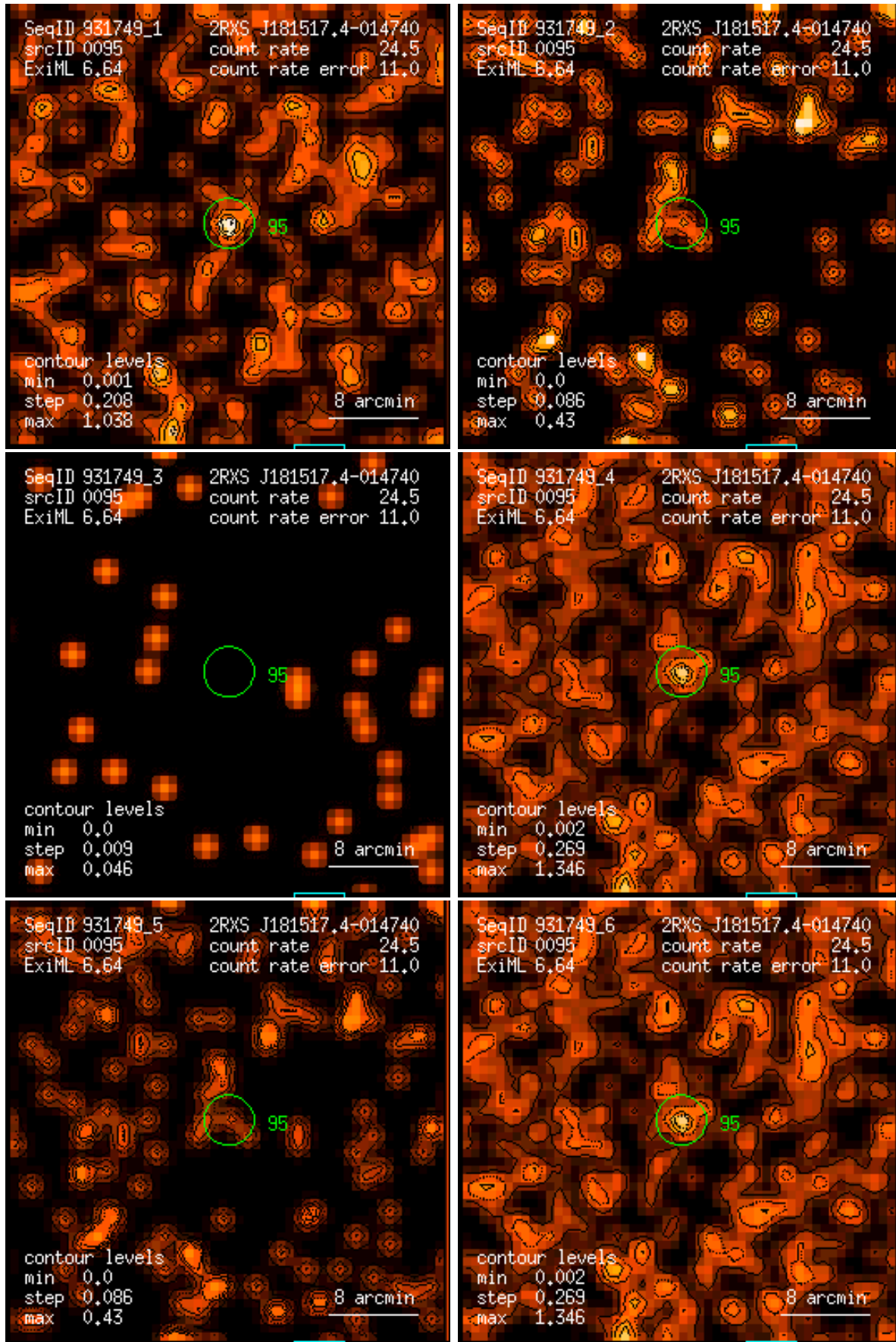
Figure 95: RASS 931749: detection 0095: band rate images, Gaussian filter: (1) PSPC channels 11 – 41, (2) 52 – 90, (3) 91 – 201, (4) 11 – 235, (5) 52 – 201, (6) 11 – 201. Broad band rates in counts/ks. Band rate contour levels in counts/ks/arcmin 2 .
