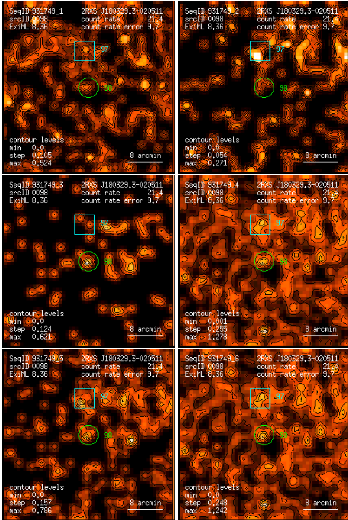
Figure 98: RASS 931749: detection 0098: band rate images, Gaussian filter: (1) PSPC channels 11 – 41, (2) 52 – 90, (3) 91 – 201, (4) 11 – 235, (5) 52 – 201, (6) 11 – 201. Broad band rates in counts/ks. Band rate contour levels in counts/ks/arcmin 2 .
