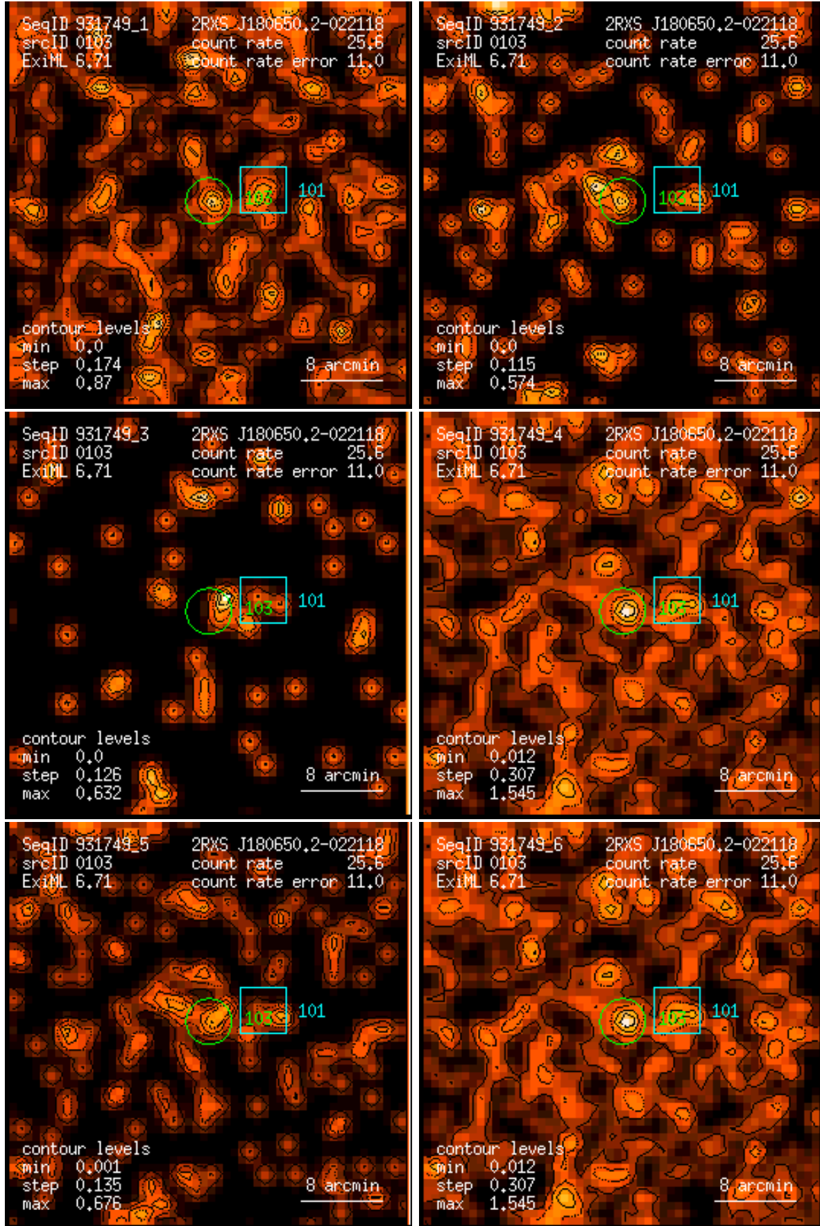
Figure 103: RASS 931749: detection 0103: band rate images, Gaussian filter: (1) PSPC channels 11 – 41, (2) 52 – 90, (3) 91 – 201, (4) 11 – 235, (5) 52 – 201, (6) 11 – 201. Broad band rates in counts/ks. Band rate contour levels in counts/ks/arcmin 2 .
