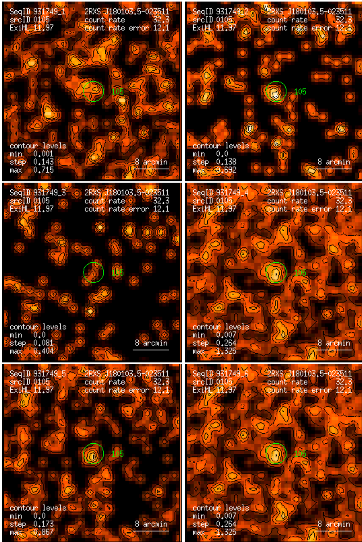
Figure 105: RASS 931749: detection 0105: band rate images, Gaussian filter: (1) PSPC channels 11 – 41, (2) 52 – 90, (3) 91 – 201, (4) 11 – 235, (5) 52 – 201, (6) 11 – 201. Broad band rates in counts/ks. Band rate contour levels in counts/ks/arcmin 2 .
