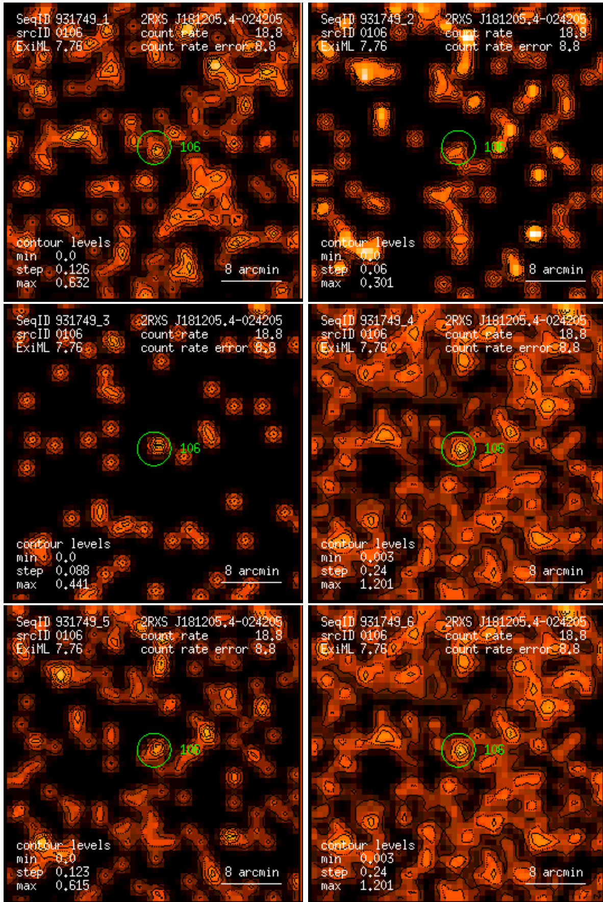
Figure 106: RASS 931749: detection 0106: band rate images, Gaussian filter: (1) PSPC channels 11 – 41, (2) 52 – 90, (3) 91 – 201, (4) 11 – 235, (5) 52 – 201, (6) 11 – 201. Broad band rates in counts/ks. Band rate contour levels in counts/ks/arcmin 2 .
