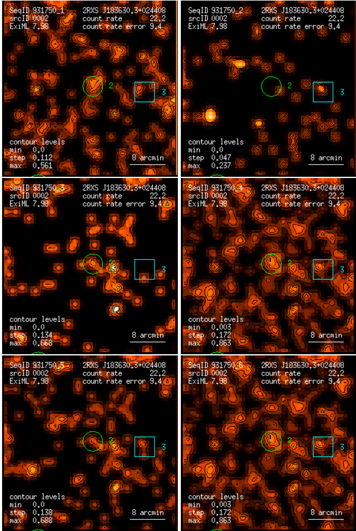
Figure 2: RASS 931750: detection 0002: band rate images, Gaussian filter: (1) PSPC channels 11 – 41, (2) 52 – 90, (3) 91 – 201, (4) 11 – 235, (5) 52 – 201, (6) 11 – 201. Broad band rates in counts/ks. Band rate contour levels in counts/ks/arcmin 2 .
