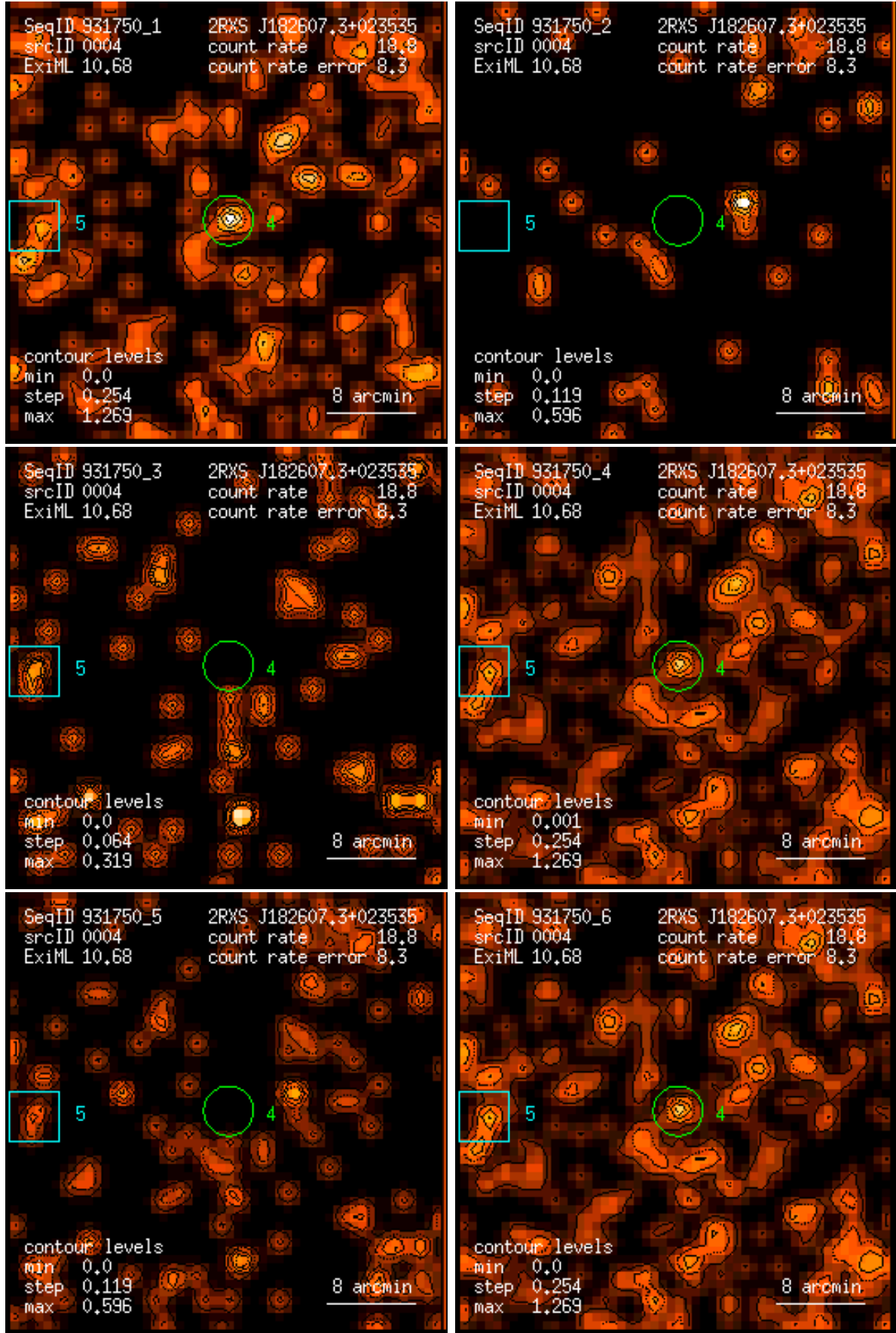
Figure 4: RASS 931750: detection 0004: band rate images, Gaussian filter: (1) PSPC channels 11 – 41, (2) 52 – 90, (3) 91 – 201, (4) 11 – 235, (5) 52 – 201, (6) 11 – 201. Broad band rates in counts/ks. Band rate contour levels in counts/ks/arcmin 2 .
