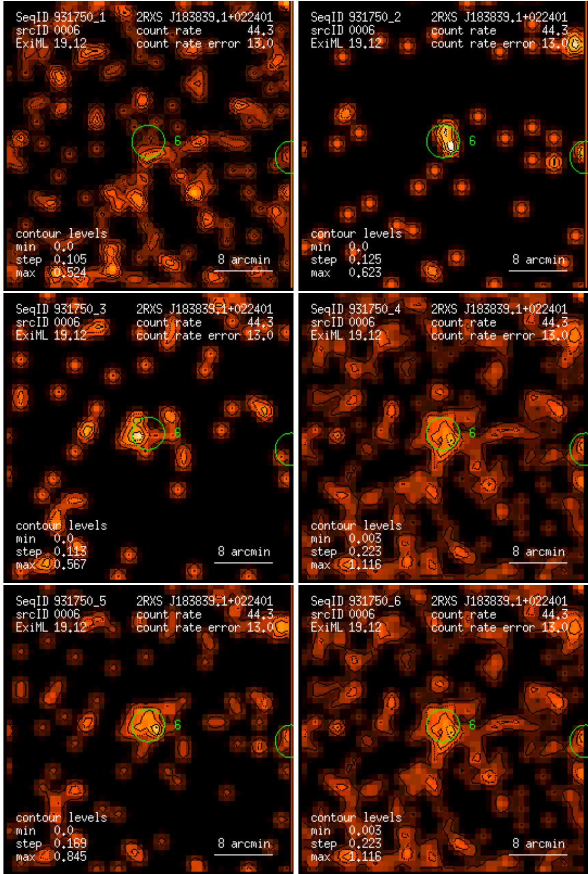
Figure 6: RASS 931750: detection 0006: band rate images, Gaussian filter: (1) PSPC channels 11 – 41, (2) 52 – 90, (3) 91 – 201, (4) 11 – 235, (5) 52 – 201, (6) 11 – 201. Broad band rates in counts/ks. Band rate contour levels in counts/ks/arcmin 2 .
