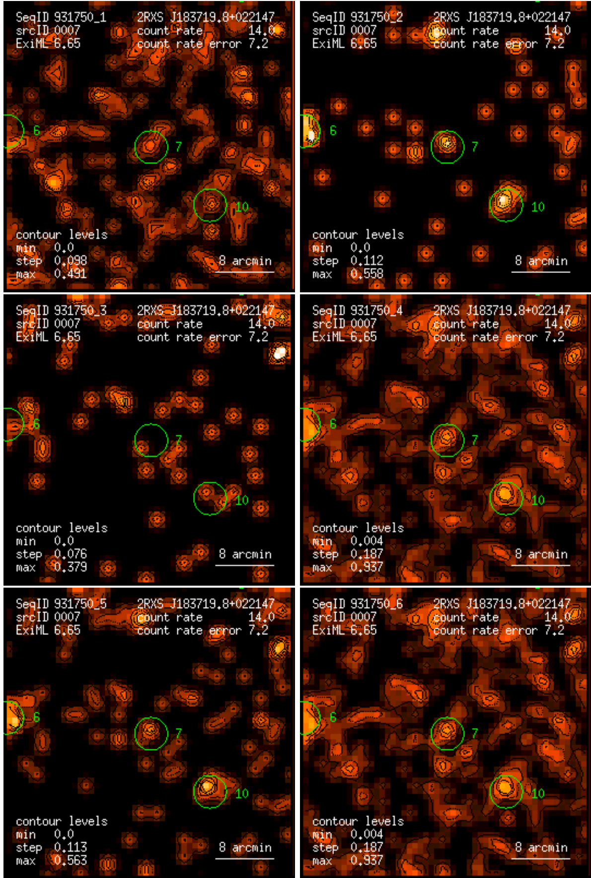
Figure 7: RASS 931750: detection 0007: band rate images, Gaussian filter: (1) PSPC channels 11 – 41, (2) 52 – 90, (3) 91 – 201, (4) 11 – 235, (5) 52 – 201, (6) 11 – 201. Broad band rates in counts/ks. Band rate contour levels in counts/ks/arcmin 2 .
