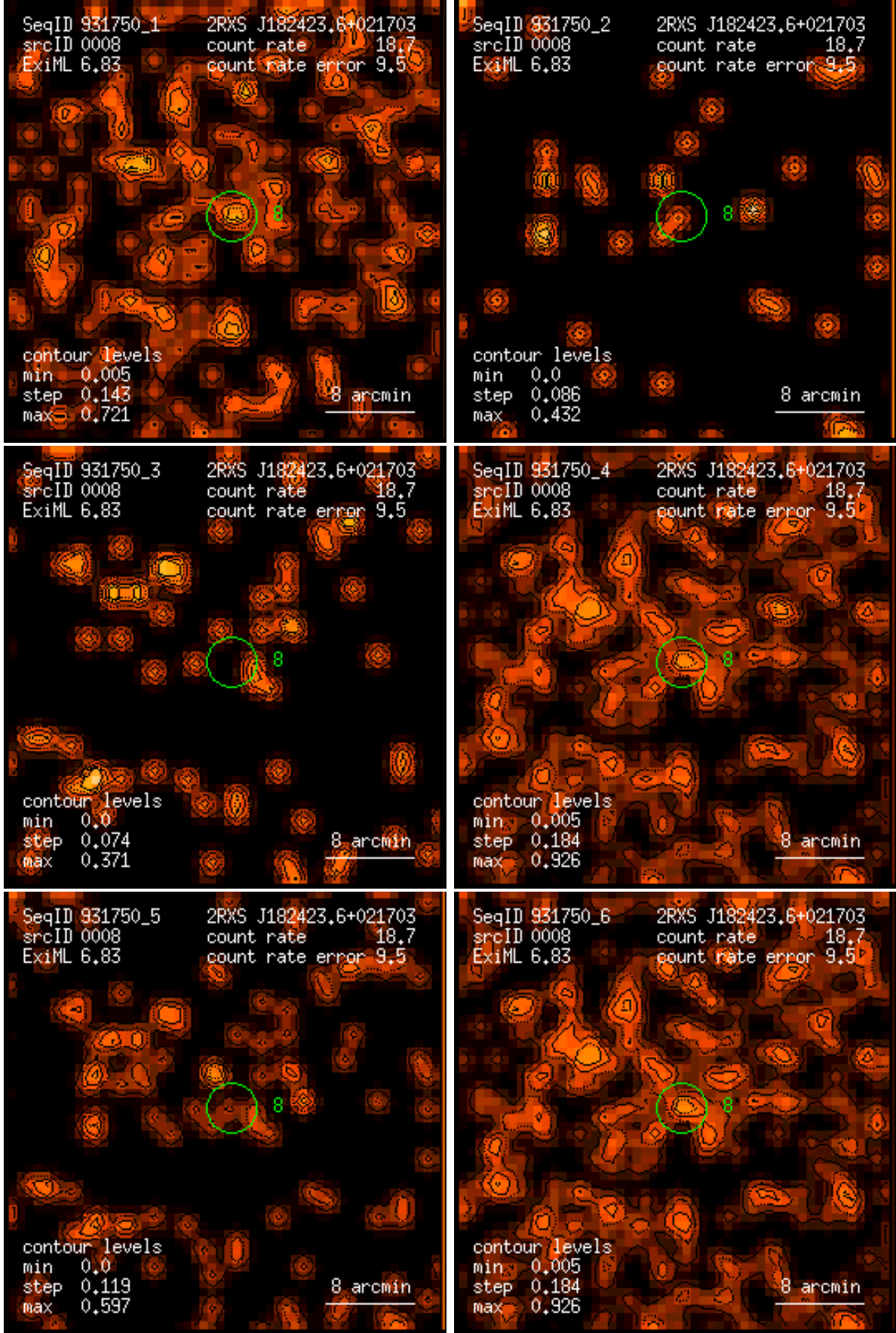
Figure 8: RASS 931750: detection 0008: band rate images, Gaussian filter: (1) PSPC channels 11 – 41, (2) 52 – 90, (3) 91 – 201, (4) 11 – 235, (5) 52 – 201, (6) 11 – 201. Broad band rates in counts/ks. Band rate contour levels in counts/ks/arcmin 2 .
