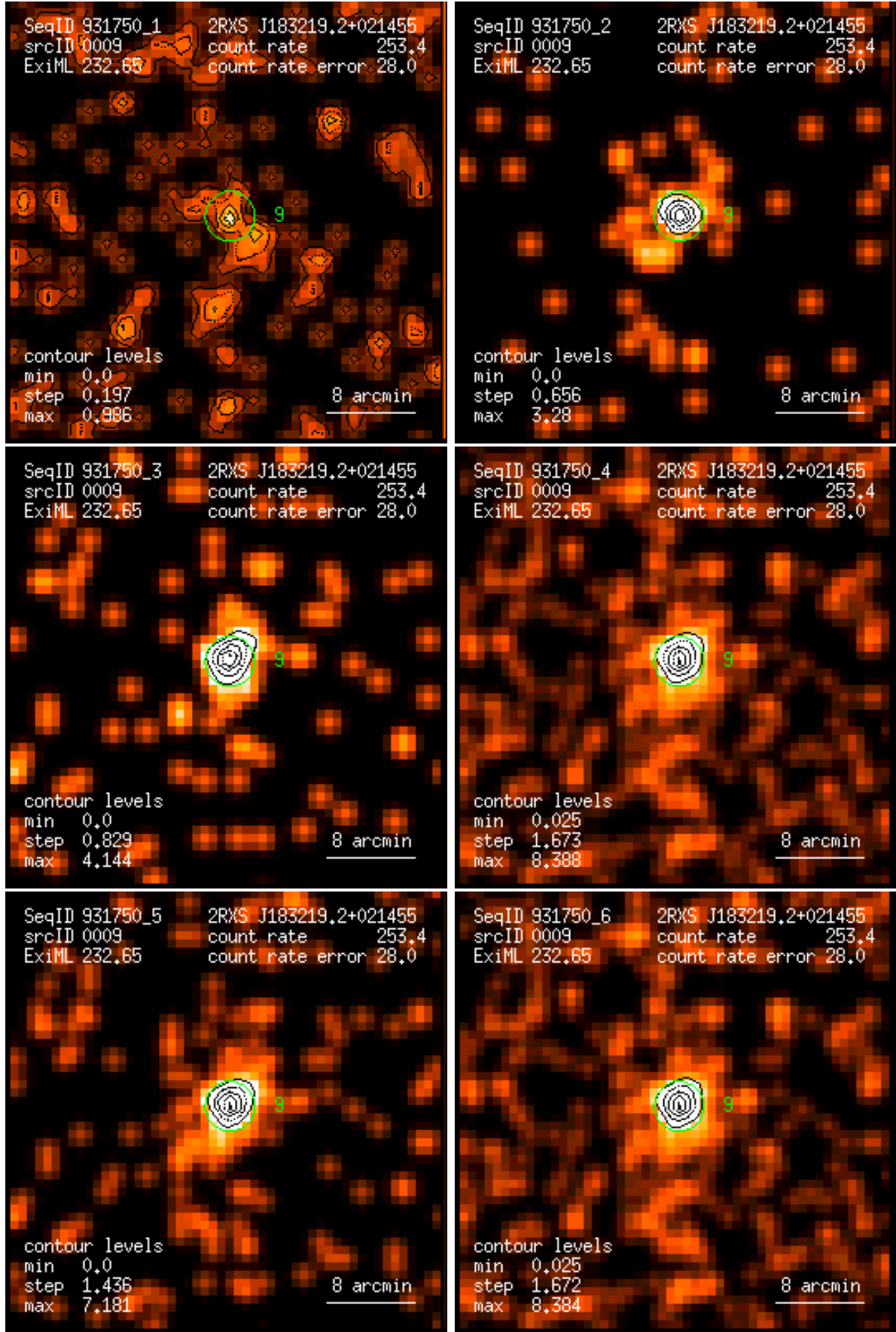
Figure 9: RASS 931750: detection 0009: band rate images, Gaussian filter: (1) PSPC channels 11 – 41, (2) 52 – 90, (3) 91 – 201, (4) 11 – 235, (5) 52 – 201, (6) 11 – 201. Broad band rates in counts/ks. Band rate contour levels in counts/ks/arcmin 2 .
