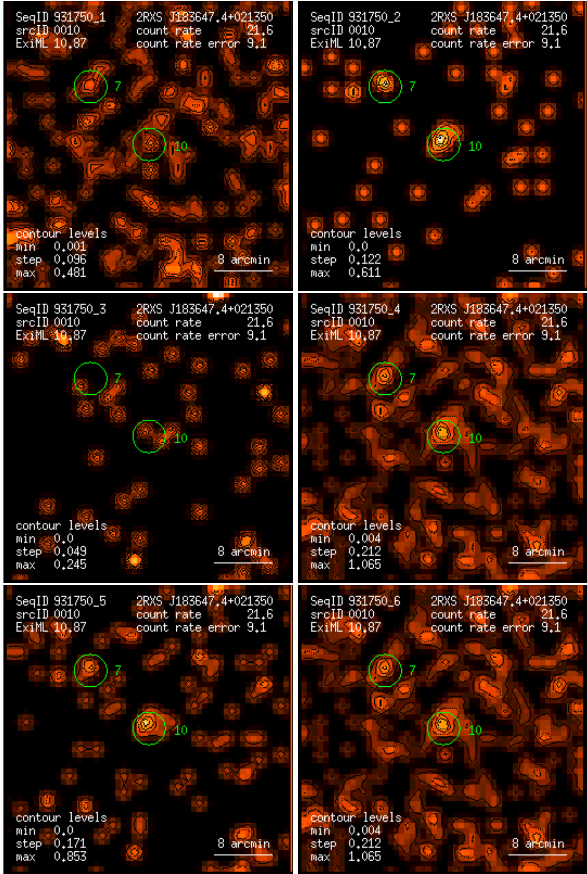
Figure 10: RASS 931750: detection 0010: band rate images, Gaussian filter: (1) PSPC channels 11 – 41, (2) 52 – 90, (3) 91 – 201, (4) 11 – 235, (5) 52 – 201, (6) 11 – 201. Broad band rates in counts/ks. Band rate contour levels in counts/ks/arcmin 2 .
