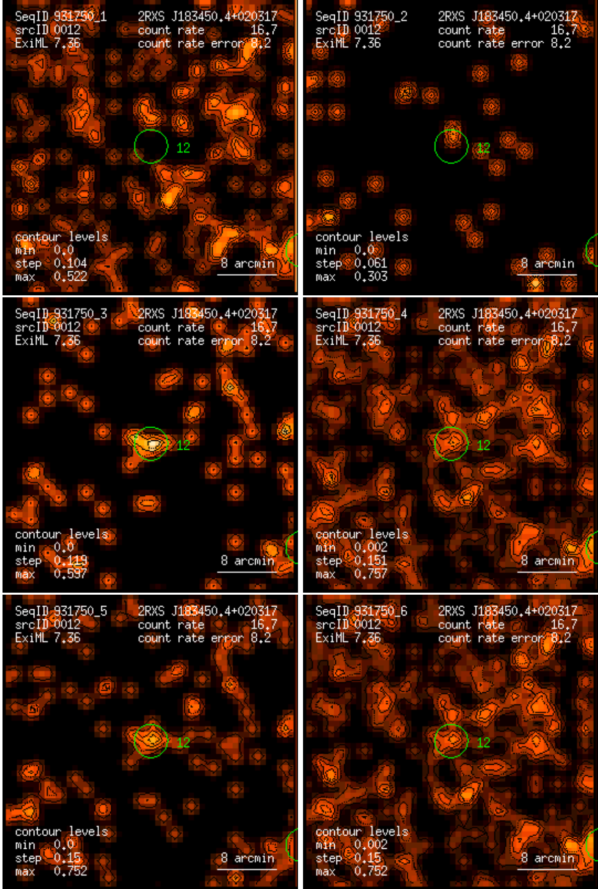
Figure 12: RASS 931750: detection 0012: band rate images, Gaussian filter: (1) PSPC channels 11 – 41, (2) 52 – 90, (3) 91 – 201, (4) 11 – 235, (5) 52 – 201, (6) 11 – 201. Broad band rates in counts/ks. Band rate contour levels in counts/ks/arcmin 2 .
