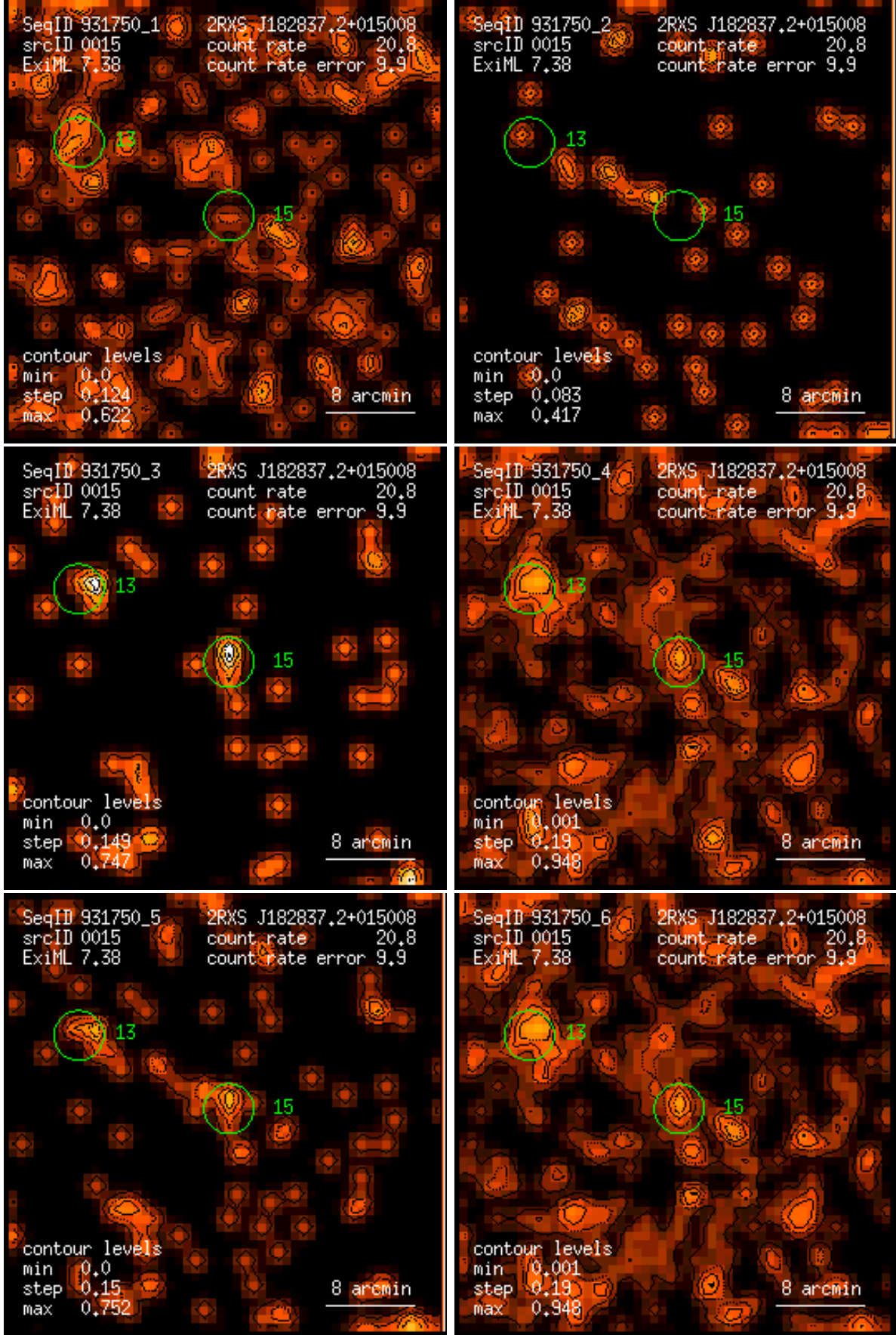
Figure 15: RASS 931750: detection 0015: band rate images, Gaussian filter: (1) PSPC channels 11 – 41, (2) 52 – 90, (3) 91 – 201, (4) 11 – 235, (5) 52 – 201, (6) 11 – 201. Broad band rates in counts/ks. Band rate contour levels in counts/ks/arcmin 2 .
