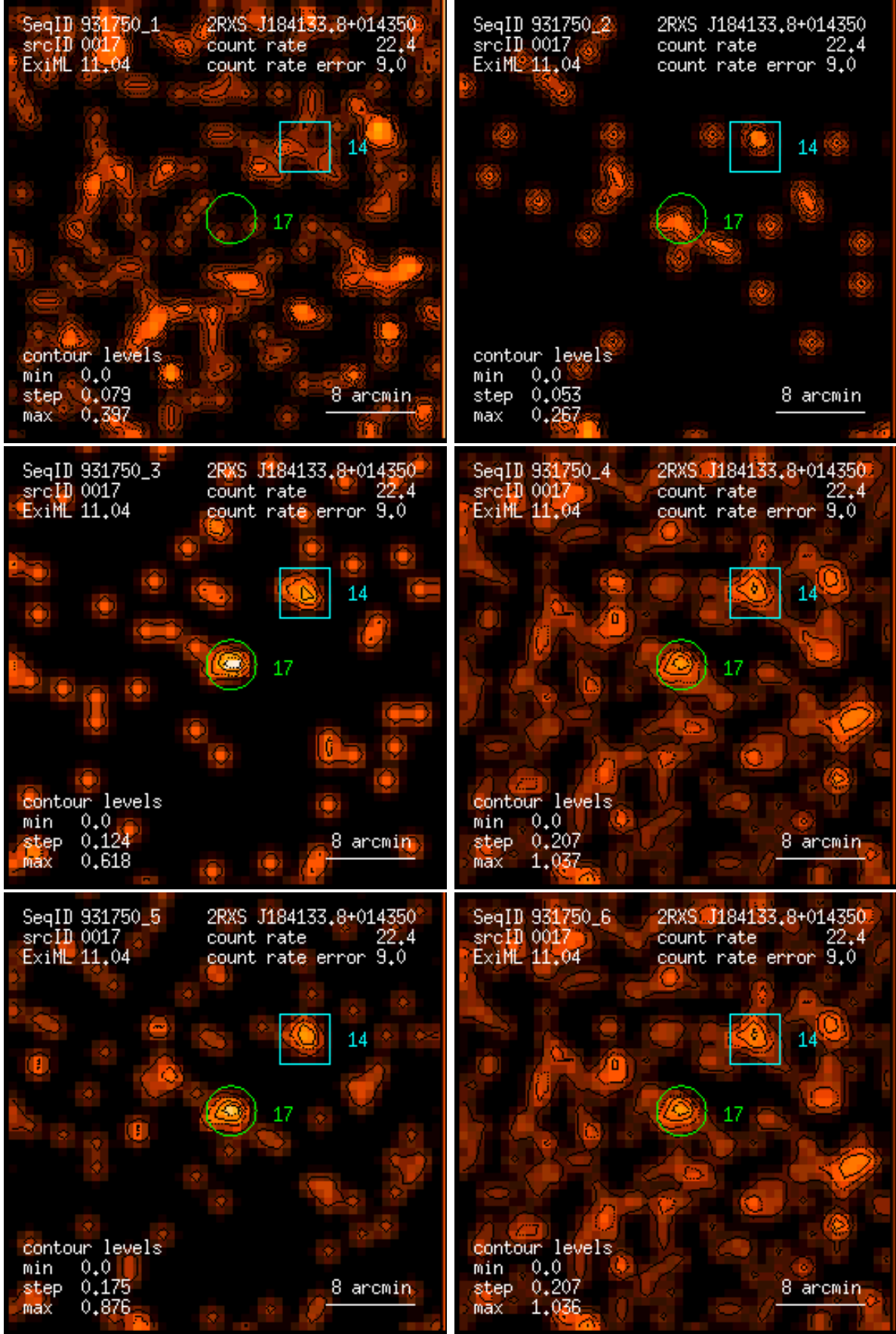
Figure 17: RASS 931750: detection 0017: band rate images, Gaussian filter: (1) PSPC channels 11 – 41, (2) 52 – 90, (3) 91 – 201, (4) 11 – 235, (5) 52 – 201, (6) 11 – 201. Broad band rates in counts/ks. Band rate contour levels in counts/ks/arcmin 2 .
