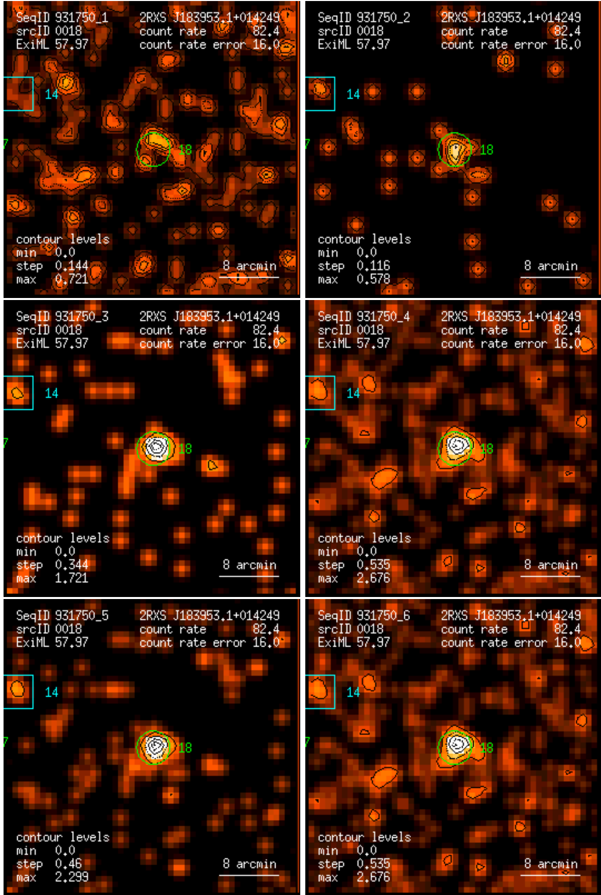
Figure 18: RASS 931750: detection 0018: band rate images, Gaussian filter: (1) PSPC channels 11 – 41, (2) 52 – 90, (3) 91 – 201, (4) 11 – 235, (5) 52 – 201, (6) 11 – 201. Broad band rates in counts/ks. Band rate contour levels in counts/ks/arcmin 2 .
