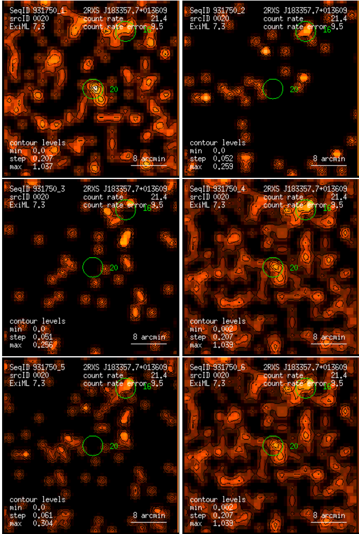
Figure 20: RASS 931750: detection 0020: band rate images, Gaussian filter: (1) PSPC channels 11 – 41, (2) 52 – 90, (3) 91 – 201, (4) 11 – 235, (5) 52 – 201, (6) 11 – 201. Broad band rates in counts/ks. Band rate contour levels in counts/ks/arcmin 2 .
