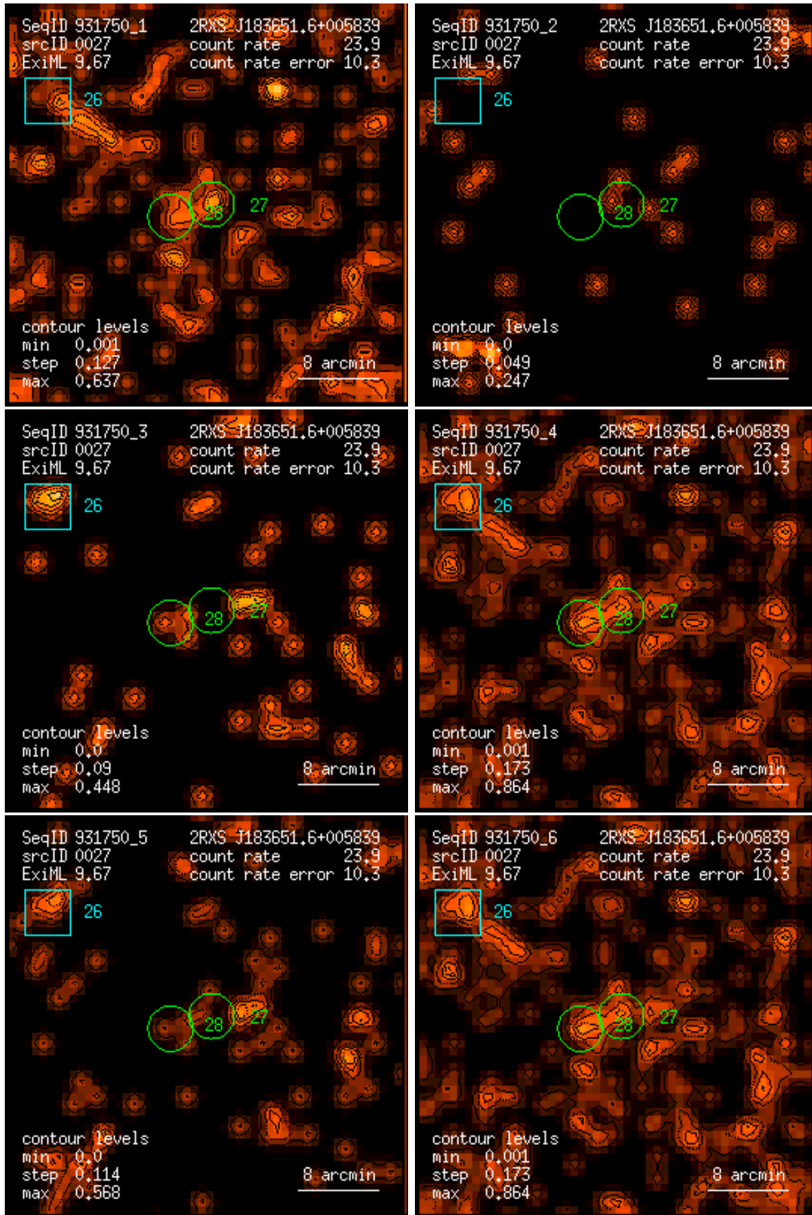
Figure 27: RASS 931750: detection 0027: band rate images, Gaussian filter: (1) PSPC channels 11 – 41, (2) 52 – 90, (3) 91 – 201, (4) 11 – 235, (5) 52 – 201, (6) 11 – 201. Broad band rates in counts/ks. Band rate contour levels in counts/ks/arcmin 2 .
