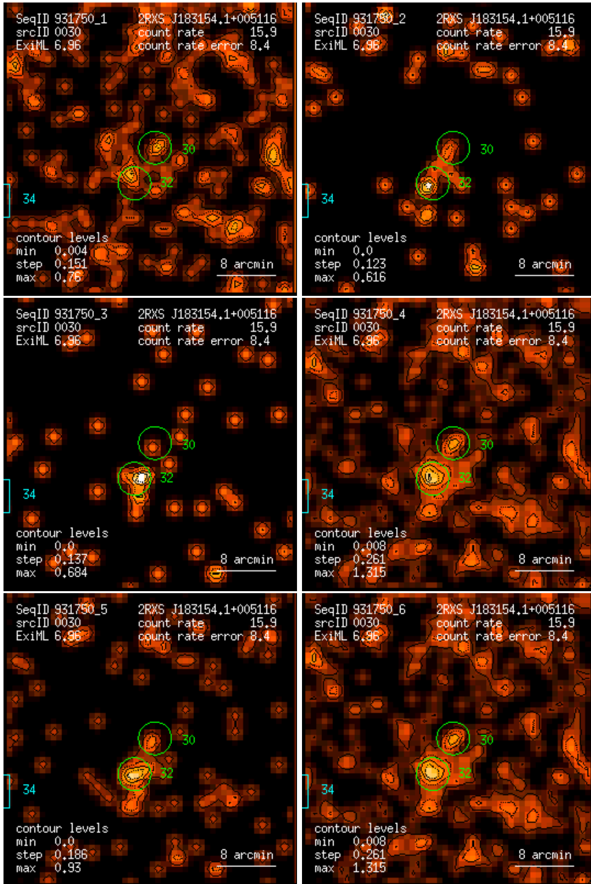
Figure 30: RASS 931750: detection 0030: band rate images, Gaussian filter: (1) PSPC channels 11 – 41, (2) 52 – 90, (3) 91 – 201, (4) 11 – 235, (5) 52 – 201, (6) 11 – 201. Broad band rates in counts/ks. Band rate contour levels in counts/ks/arcmin 2 .
