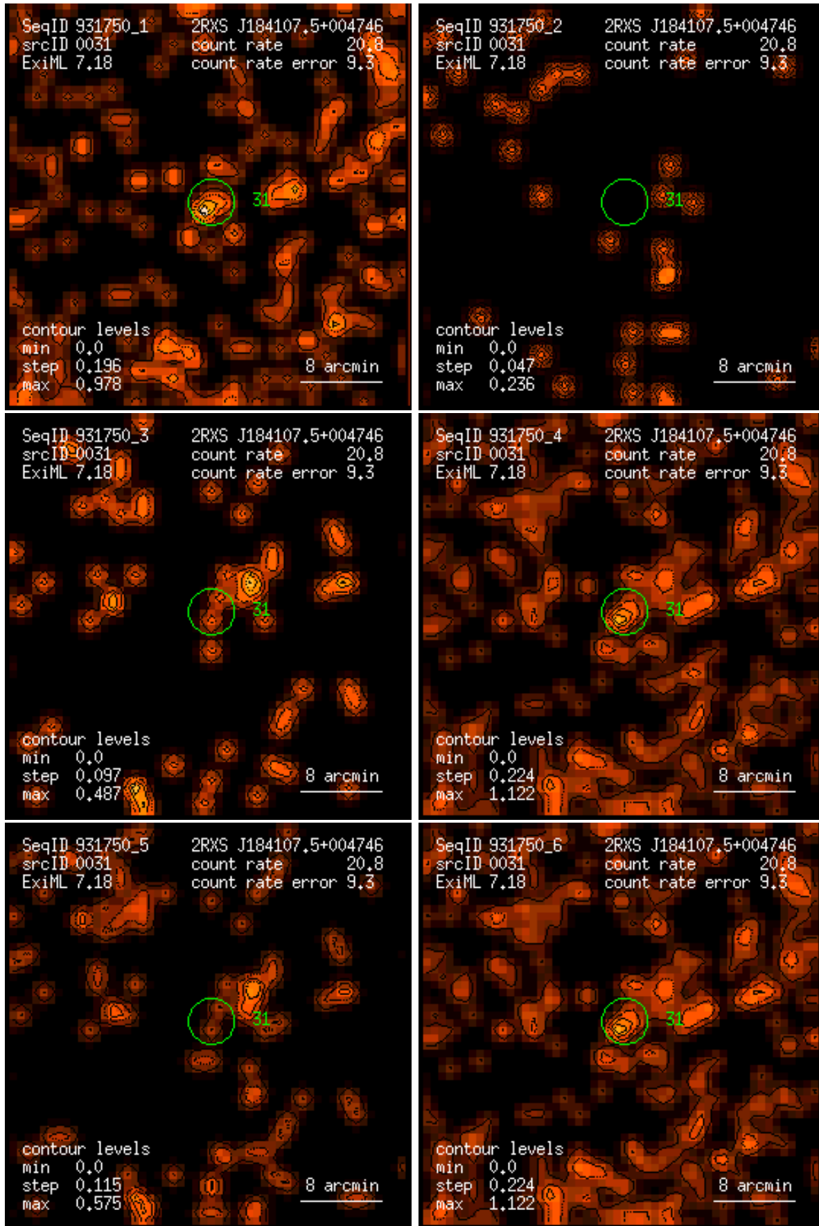
Figure 31: RASS 931750: detection 0031: band rate images, Gaussian filter: (1) PSPC channels 11 – 41, (2) 52 – 90, (3) 91 – 201, (4) 11 – 235, (5) 52 – 201, (6) 11 – 201. Broad band rates in counts/ks. Band rate contour levels in counts/ks/arcmin 2 .
