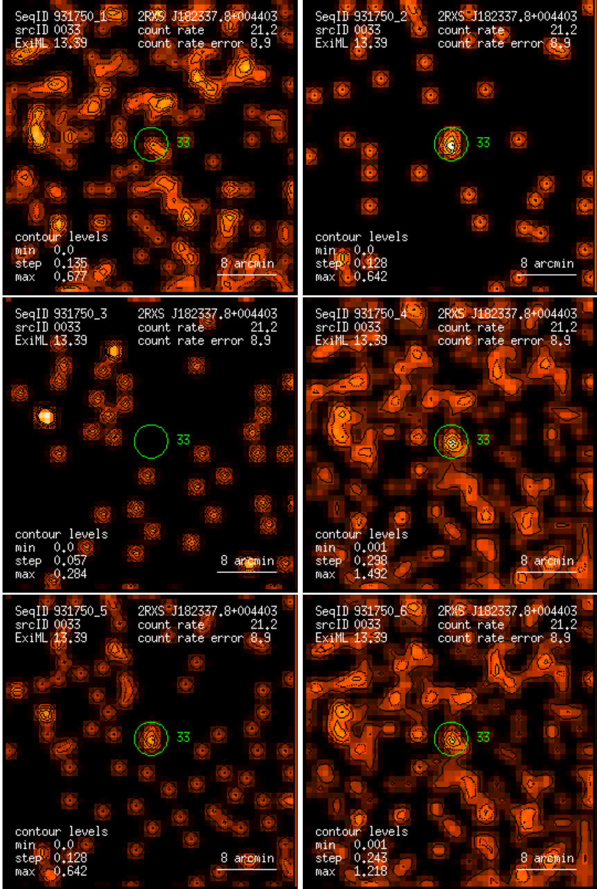
Figure 33: RASS 931750: detection 0033: band rate images, Gaussian filter: (1) PSPC channels 11 – 41, (2) 52 – 90, (3) 91 – 201, (4) 11 – 235, (5) 52 – 201, (6) 11 – 201. Broad band rates in counts/ks. Band rate contour levels in counts/ks/arcmin 2 .
