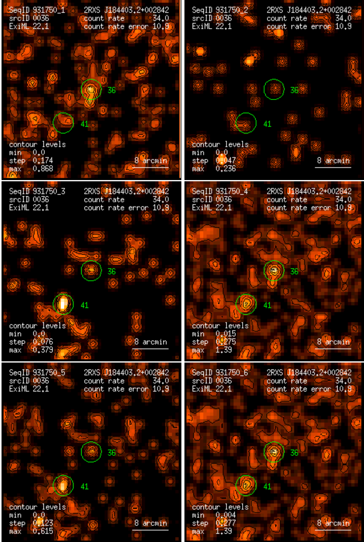
Figure 36: RASS 931750: detection 0036: band rate images, Gaussian filter: (1) PSPC channels 11 – 41, (2) 52 – 90, (3) 91 – 201, (4) 11 – 235, (5) 52 – 201, (6) 11 – 201. Broad band rates in counts/ks. Band rate contour levels in counts/ks/arcmin 2 .
