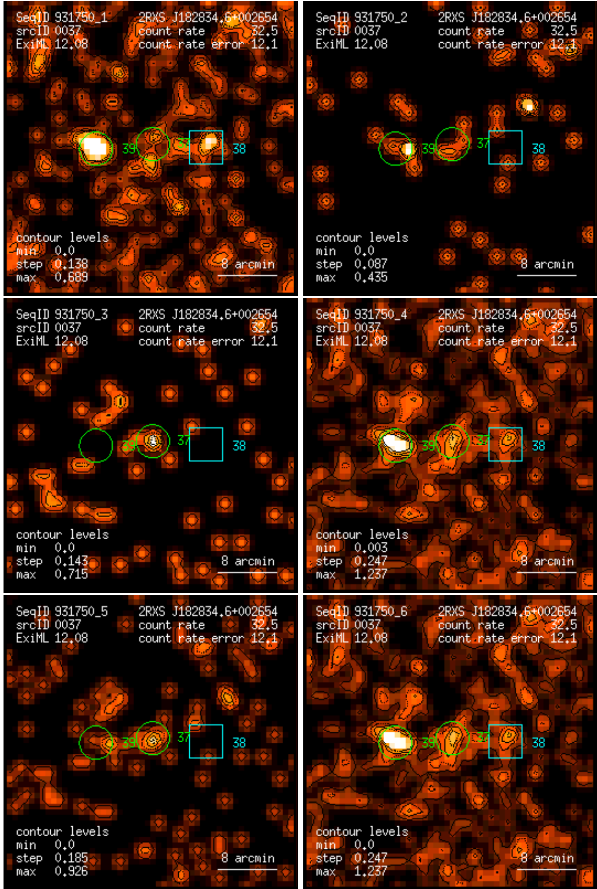
Figure 37: RASS 931750: detection 0037: band rate images, Gaussian filter: (1) PSPC channels 11 – 41, (2) 52 – 90, (3) 91 – 201, (4) 11 – 235, (5) 52 – 201, (6) 11 – 201. Broad band rates in counts/ks. Band rate contour levels in counts/ks/arcmin 2 .
