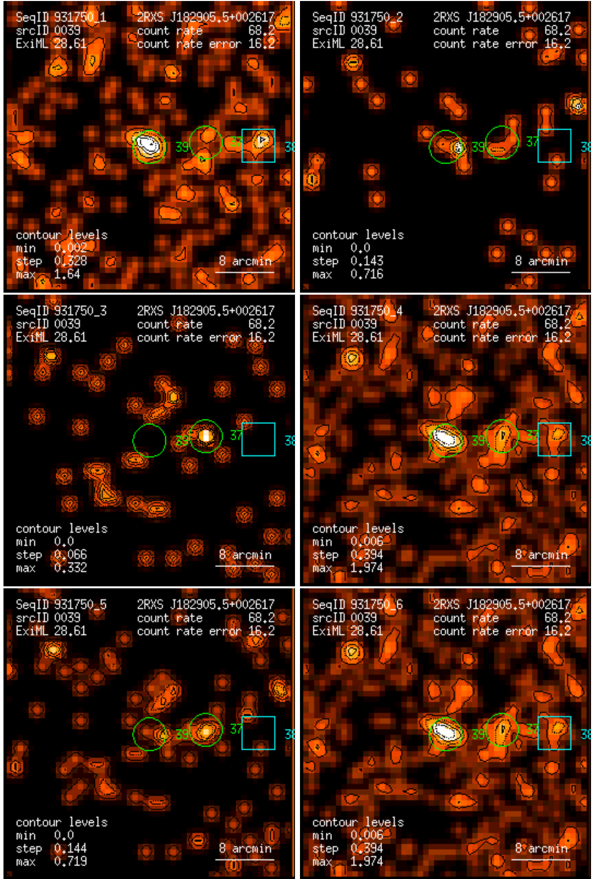
Figure 39: RASS 931750: detection 0039: band rate images, Gaussian filter: (1) PSPC channels 11 – 41, (2) 52 – 90, (3) 91 – 201, (4) 11 – 235, (5) 52 – 201, (6) 11 – 201. Broad band rates in counts/ks. Band rate contour levels in counts/ks/arcmin 2 .
