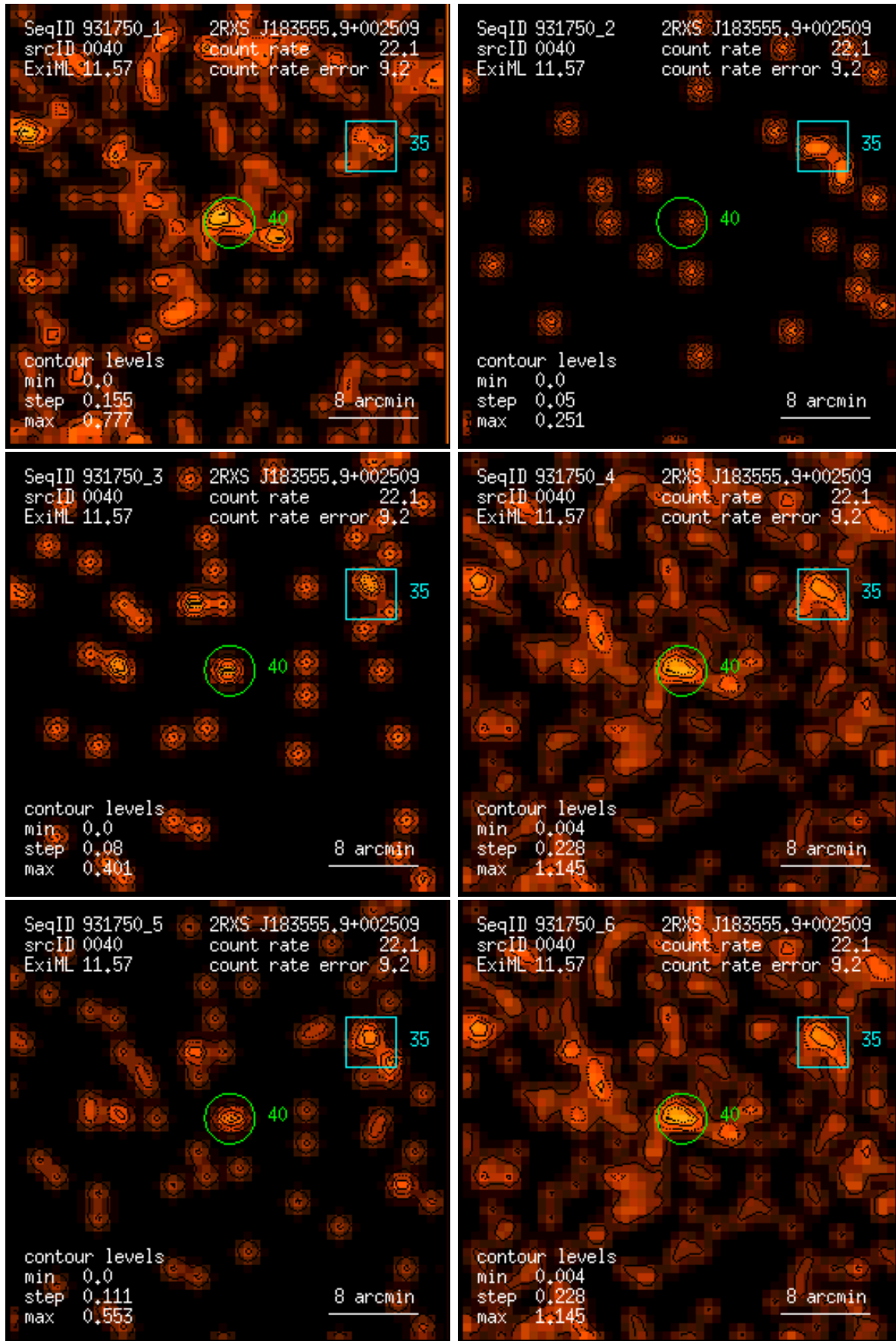
Figure 40: RASS 931750: detection 0040: band rate images, Gaussian filter: (1) PSPC channels 11 – 41, (2) 52 – 90, (3) 91 – 201, (4) 11 – 235, (5) 52 – 201, (6) 11 – 201. Broad band rates in counts/ks. Band rate contour levels in counts/ks/arcmin 2 .
