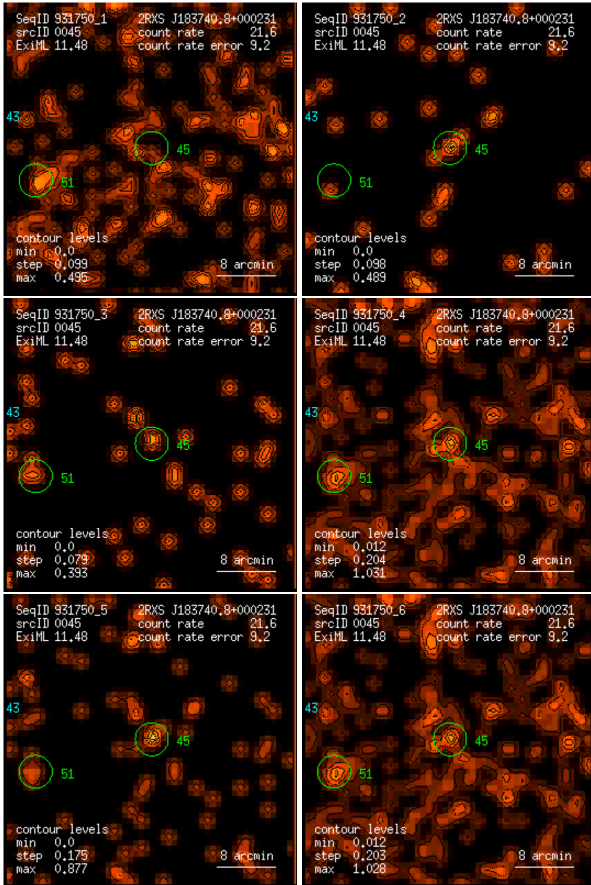
Figure 45: RASS 931750: detection 0045: band rate images, Gaussian filter: (1) PSPC channels 11 – 41, (2) 52 – 90, (3) 91 – 201, (4) 11 – 235, (5) 52 – 201, (6) 11 – 201. Broad band rates in counts/ks. Band rate contour levels in counts/ks/arcmin 2 .
