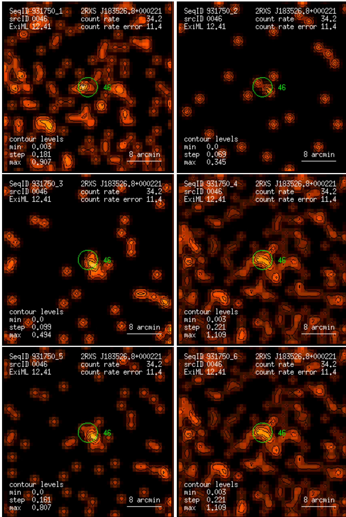
Figure 46: RASS 931750: detection 0046: band rate images, Gaussian filter: (1) PSPC channels 11 – 41, (2) 52 – 90, (3) 91 – 201, (4) 11 – 235, (5) 52 – 201, (6) 11 – 201. Broad band rates in counts/ks. Band rate contour levels in counts/ks/arcmin 2 .
