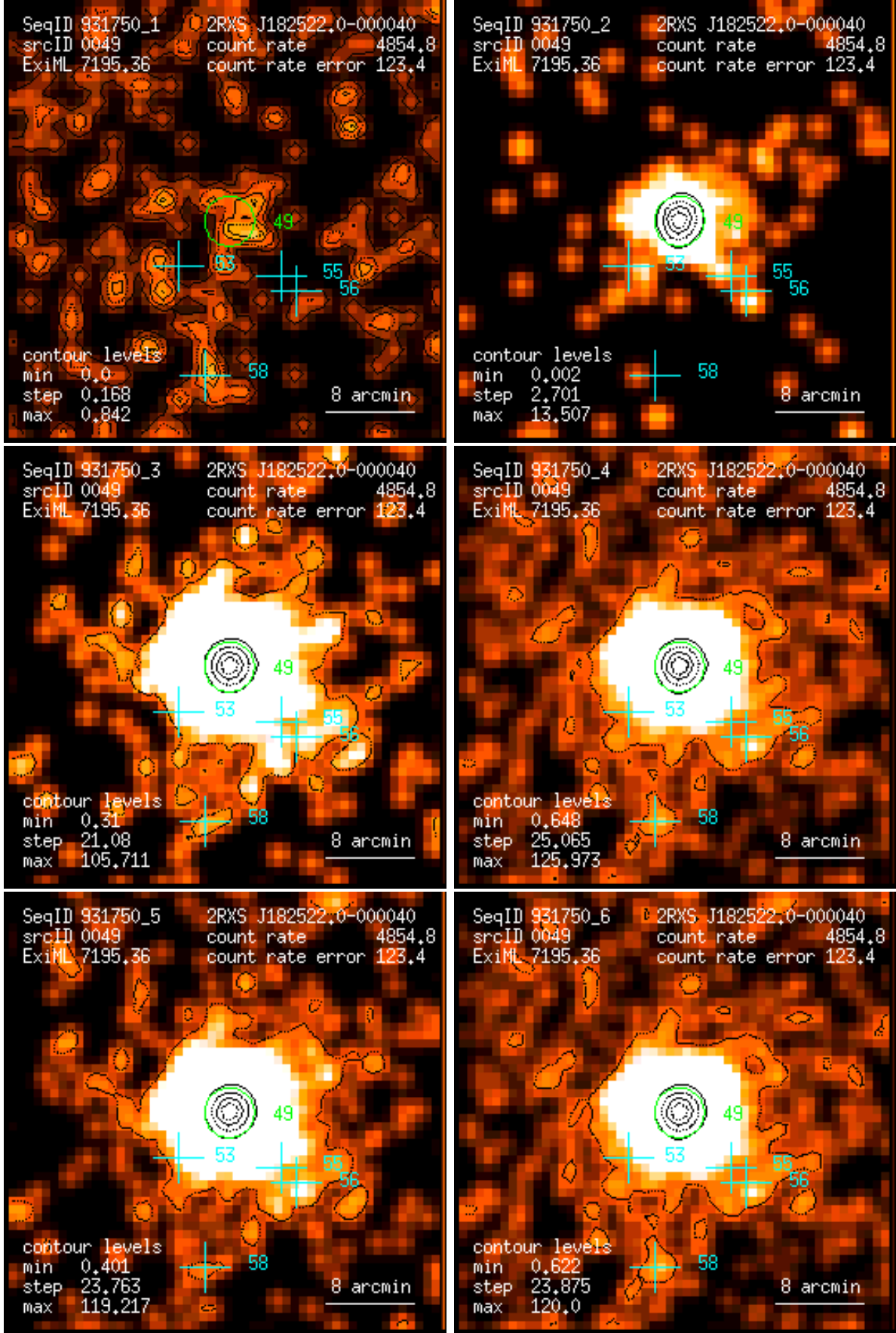
Figure 49: RASS 931750: detection 0049: band rate images, Gaussian filter: (1) PSPC channels 11 – 41, (2) 52 – 90, (3) 91 – 201, (4) 11 – 235, (5) 52 – 201, (6) 11 – 201. Broad band rates in counts/ks. Band rate contour levels in counts/ks/arcmin 2 .
