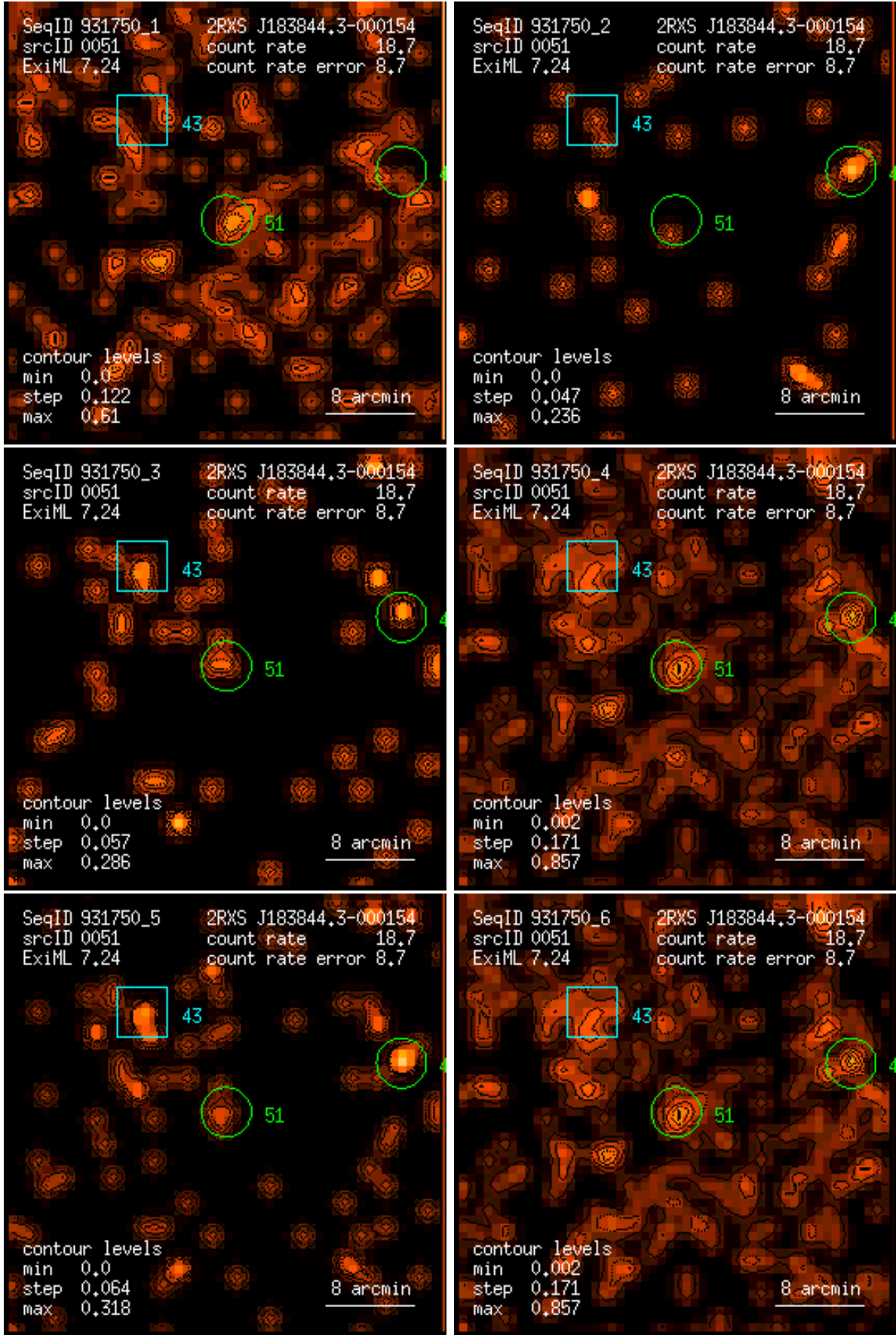
Figure 51: RASS 931750: detection 0051: band rate images, Gaussian filter: (1) PSPC channels 11 – 41, (2) 52 – 90, (3) 91 – 201, (4) 11 – 235, (5) 52 – 201, (6) 11 – 201. Broad band rates in counts/ks. Band rate contour levels in counts/ks/arcmin 2 .
