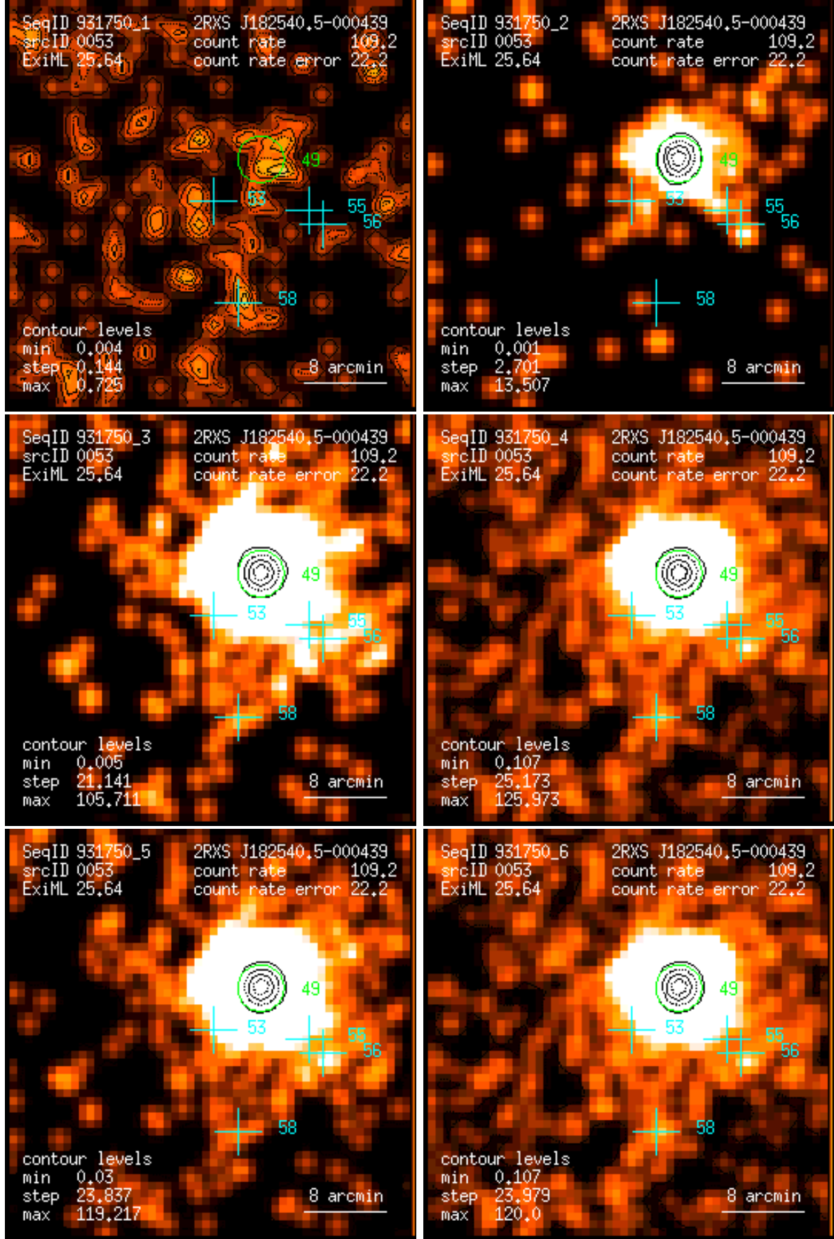
Figure 53: RASS 931750: detection 0053: band rate images, Gaussian filter: (1) PSPC channels 11 – 41, (2) 52 – 90, (3) 91 – 201, (4) 11 – 235, (5) 52 – 201, (6) 11 – 201. Broad band rates in counts/ks. Band rate contour levels in counts/ks/arcmin 2 .
