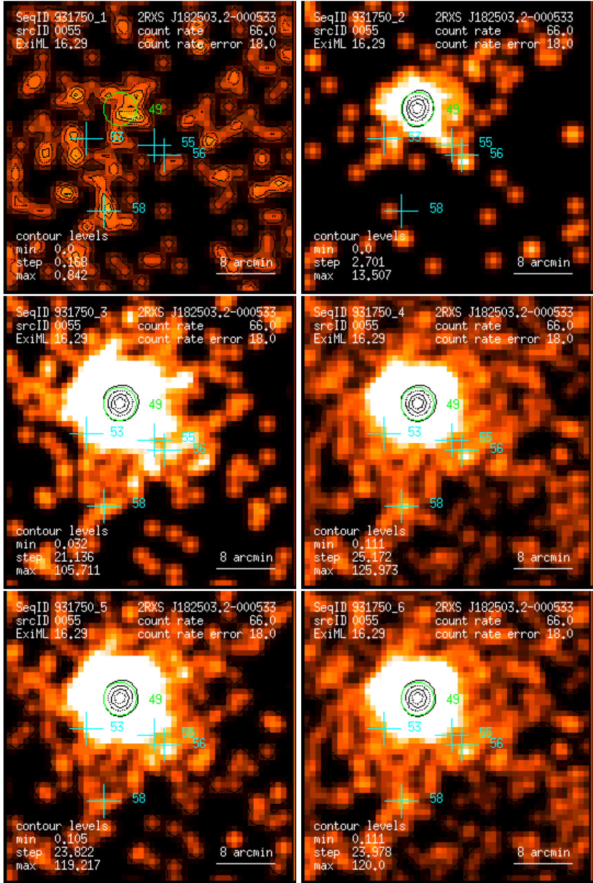
Figure 55: RASS 931750: detection 0055: band rate images, Gaussian filter: (1) PSPC channels 11 – 41, (2) 52 – 90, (3) 91 – 201, (4) 11 – 235, (5) 52 – 201, (6) 11 – 201. Broad band rates in counts/ks. Band rate contour levels in counts/ks/arcmin 2 .
