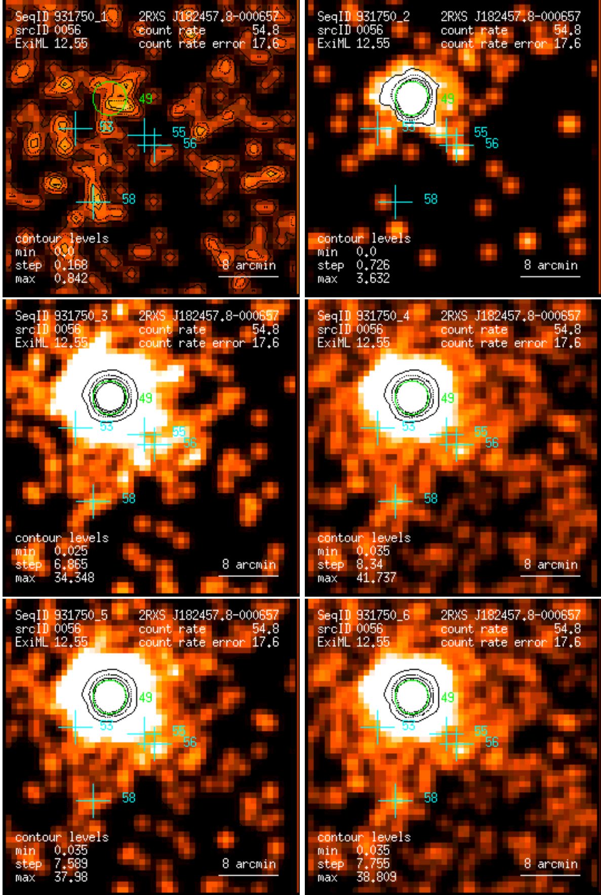
Figure 56: RASS 931750: detection 0056: band rate images, Gaussian filter: (1) PSPC channels 11 – 41, (2) 52 – 90, (3) 91 – 201, (4) 11 – 235, (5) 52 – 201, (6) 11 – 201. Broad band rates in counts/ks. Band rate contour levels in counts/ks/arcmin 2 .
