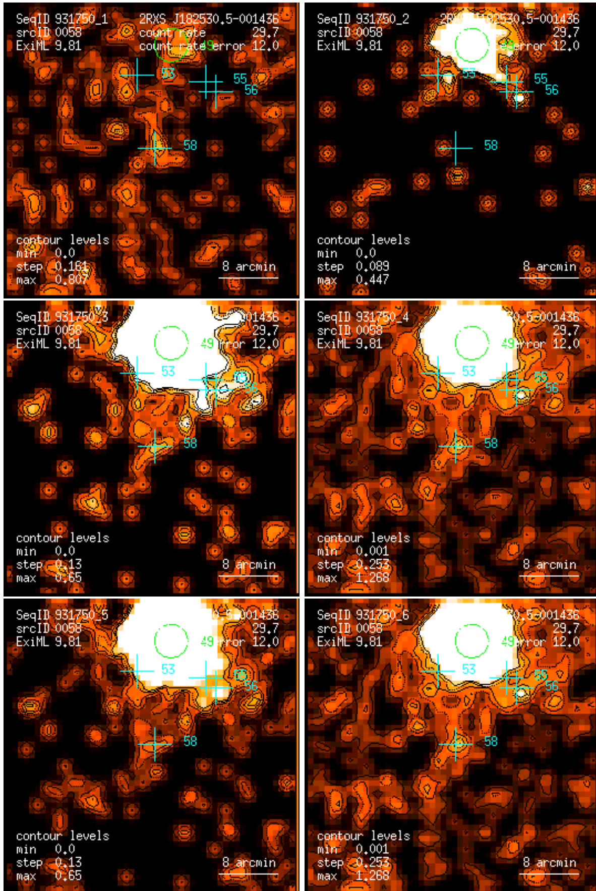
Figure 58: RASS 931750: detection 0058: band rate images, Gaussian filter: (1) PSPC channels 11 – 41, (2) 52 – 90, (3) 91 – 201, (4) 11 – 235, (5) 52 – 201, (6) 11 – 201. Broad band rates in counts/ks. Band rate contour levels in counts/ks/arcmin 2 .
