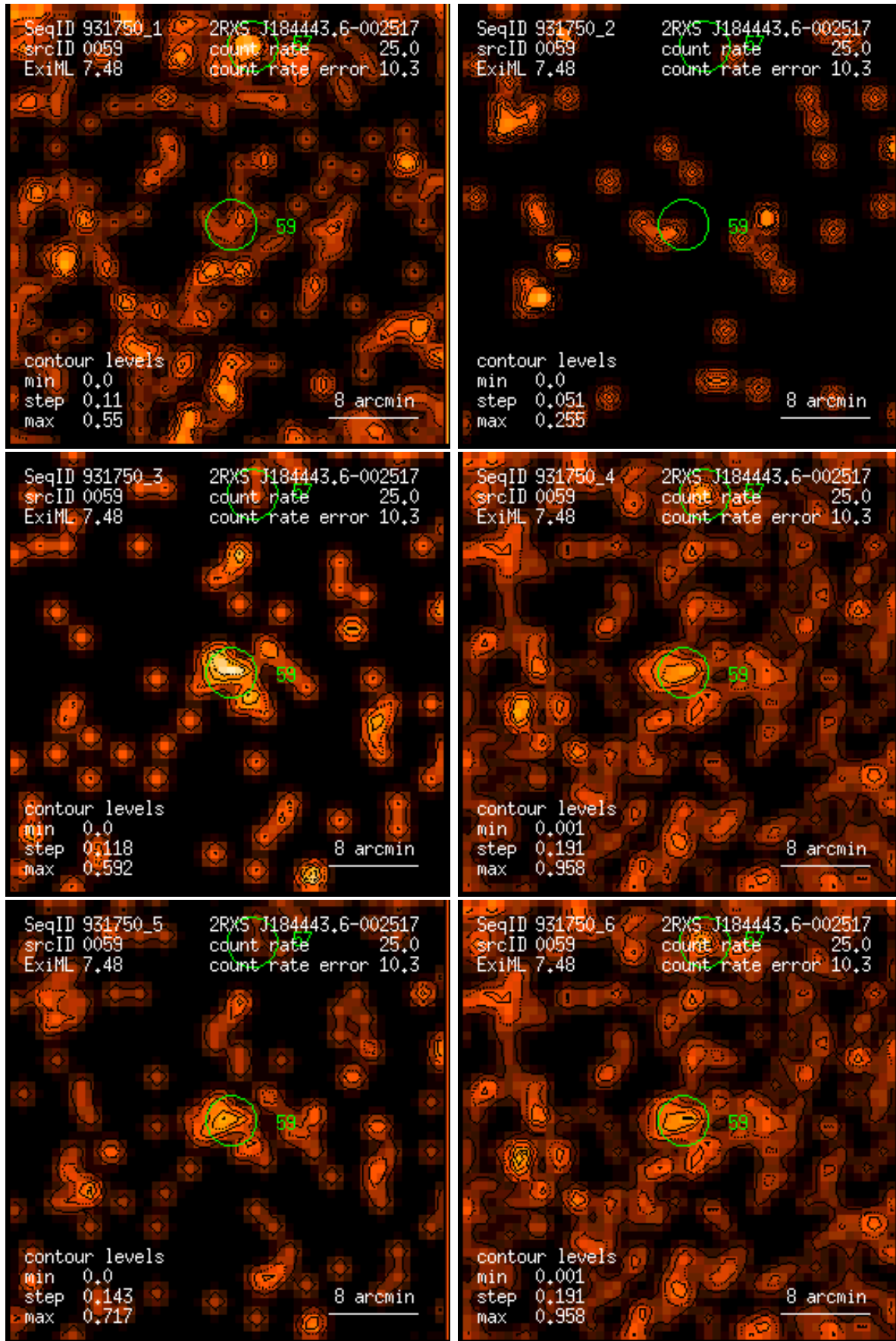
Figure 59: RASS 931750: detection 0059: band rate images, Gaussian filter: (1) PSPC channels 11 – 41, (2) 52 – 90, (3) 91 – 201, (4) 11 – 235, (5) 52 – 201, (6) 11 – 201. Broad band rates in counts/ks. Band rate contour levels in counts/ks/arcmin 2 .
