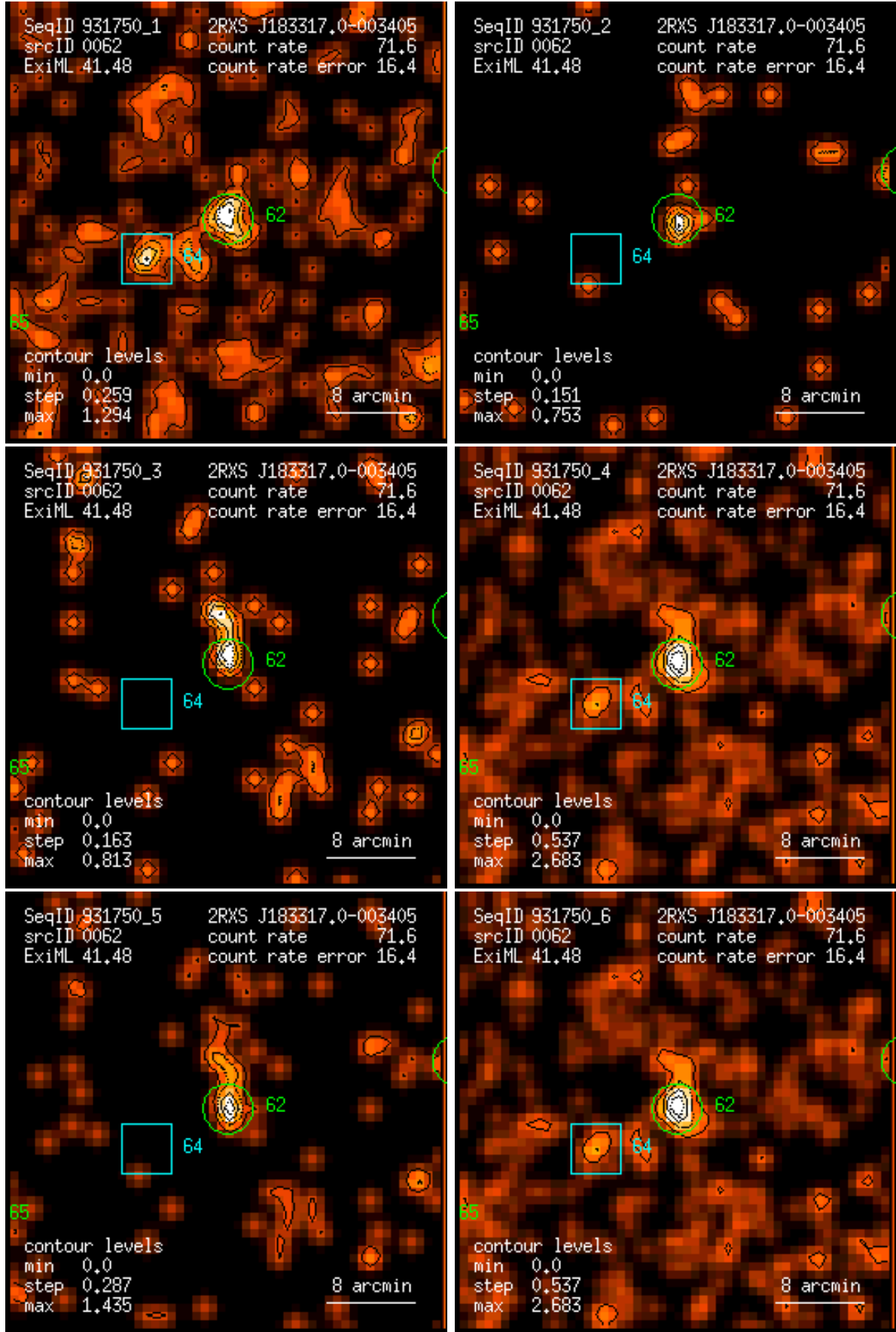
Figure 62: RASS 931750: detection 0062: band rate images, Gaussian filter: (1) PSPC channels 11 – 41, (2) 52 – 90, (3) 91 – 201, (4) 11 – 235, (5) 52 – 201, (6) 11 – 201. Broad band rates in counts/ks. Band rate contour levels in counts/ks/arcmin 2 .
