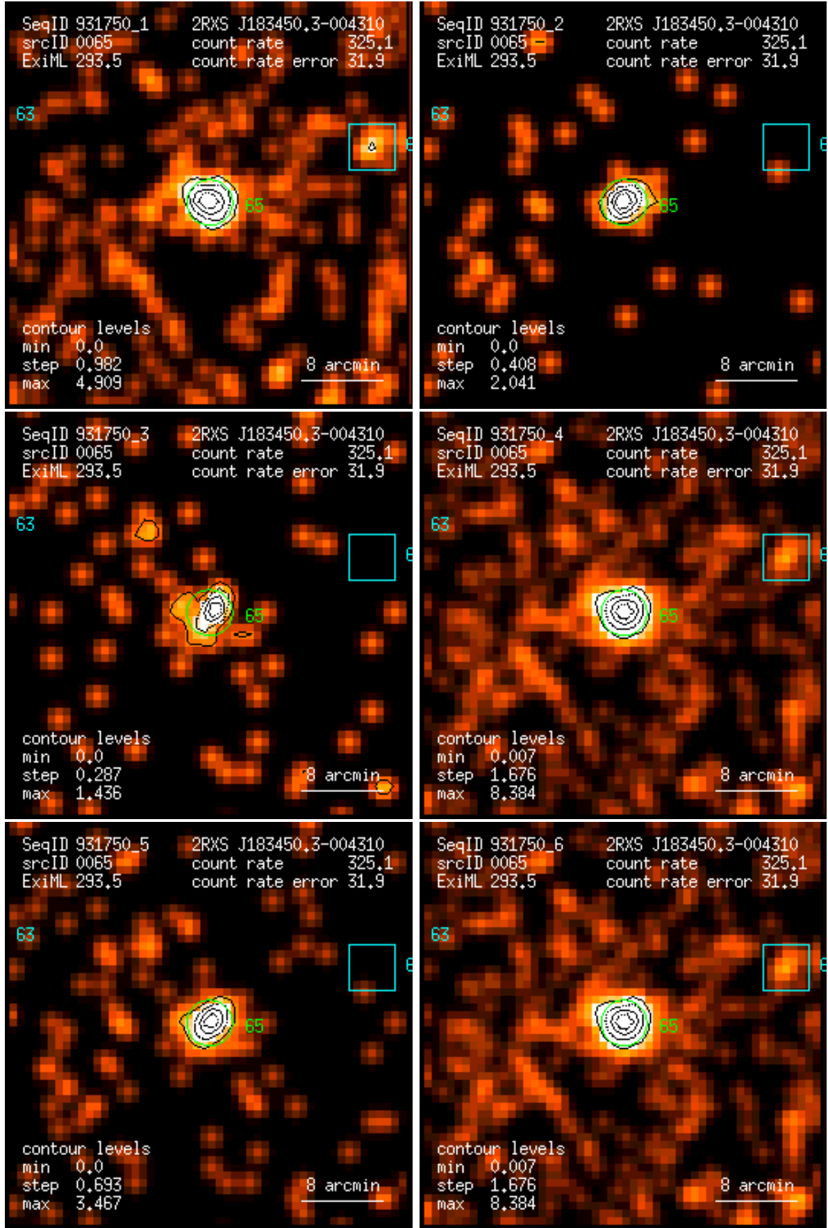
Figure 65: RASS 931750: detection 0065: band rate images, Gaussian filter: (1) PSPC channels 11 – 41, (2) 52 – 90, (3) 91 – 201, (4) 11 – 235, (5) 52 – 201, (6) 11 – 201. Broad band rates in counts/ks. Band rate contour levels in counts/ks/arcmin 2 .
