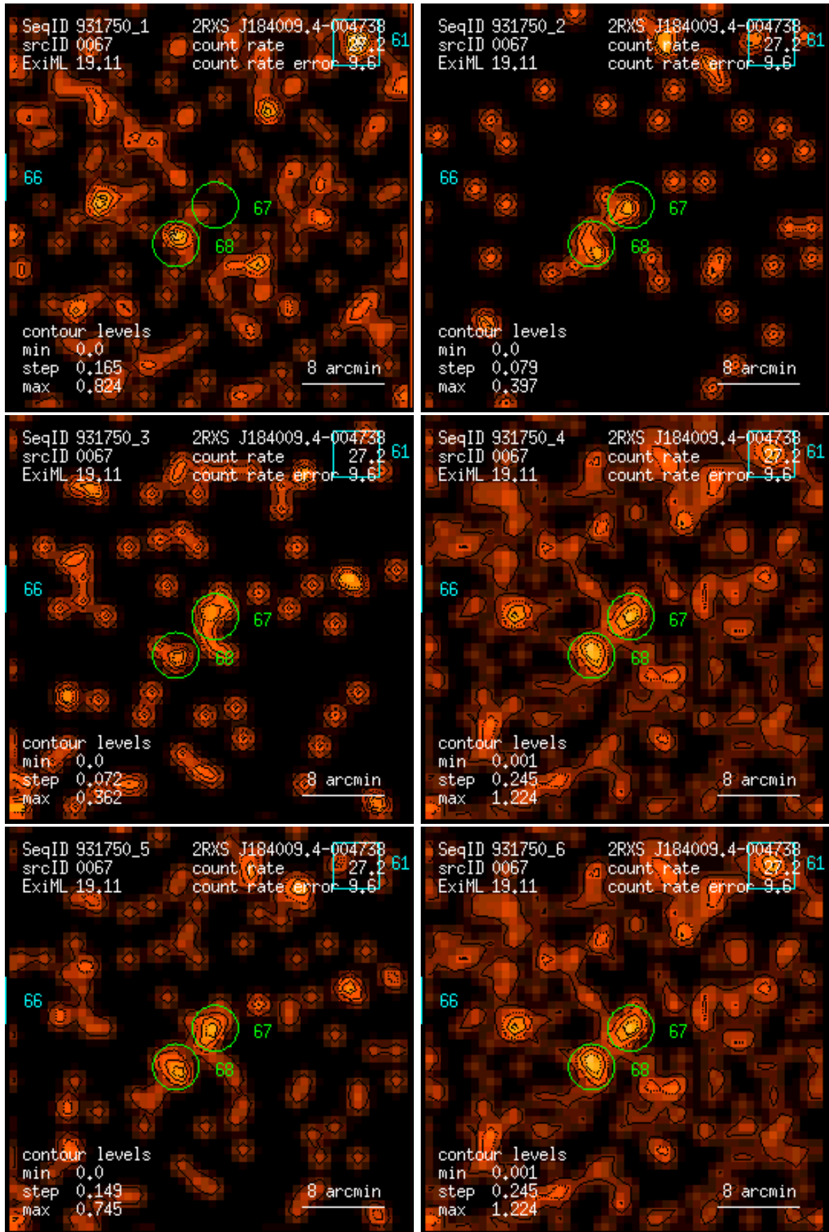
Figure 67: RASS 931750: detection 0067: band rate images, Gaussian filter: (1) PSPC channels 11 – 41, (2) 52 – 90, (3) 91 – 201, (4) 11 – 235, (5) 52 – 201, (6) 11 – 201. Broad band rates in counts/ks. Band rate contour levels in counts/ks/arcmin 2 .
