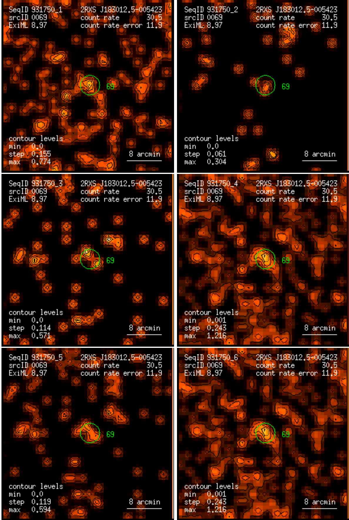
Figure 69: RASS 931750: detection 0069: band rate images, Gaussian filter: (1) PSPC channels 11 – 41, (2) 52 – 90, (3) 91 – 201, (4) 11 – 235, (5) 52 – 201, (6) 11 – 201. Broad band rates in counts/ks. Band rate contour levels in counts/ks/arcmin 2 .
