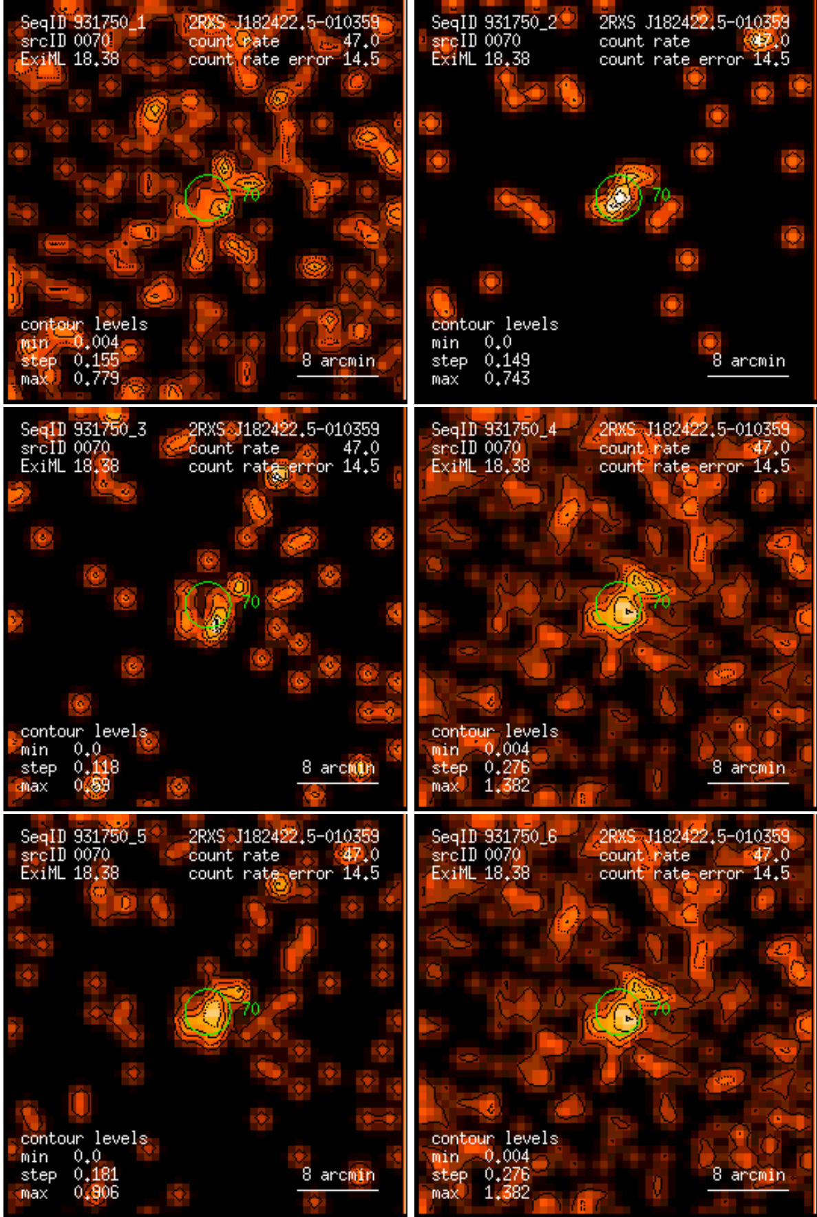
Figure 70: RASS 931750: detection 0070: band rate images, Gaussian filter: (1) PSPC channels 11 – 41, (2) 52 – 90, (3) 91 – 201, (4) 11 – 235, (5) 52 – 201, (6) 11 – 201. Broad band rates in counts/ks. Band rate contour levels in counts/ks/arcmin 2 .
