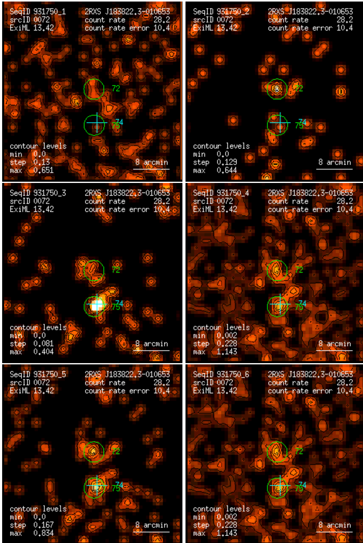
Figure 72: RASS 931750: detection 0072: band rate images, Gaussian filter: (1) PSPC channels 11 – 41, (2) 52 – 90, (3) 91 – 201, (4) 11 – 235, (5) 52 – 201, (6) 11 – 201. Broad band rates in counts/ks. Band rate contour levels in counts/ks/arcmin 2 .
