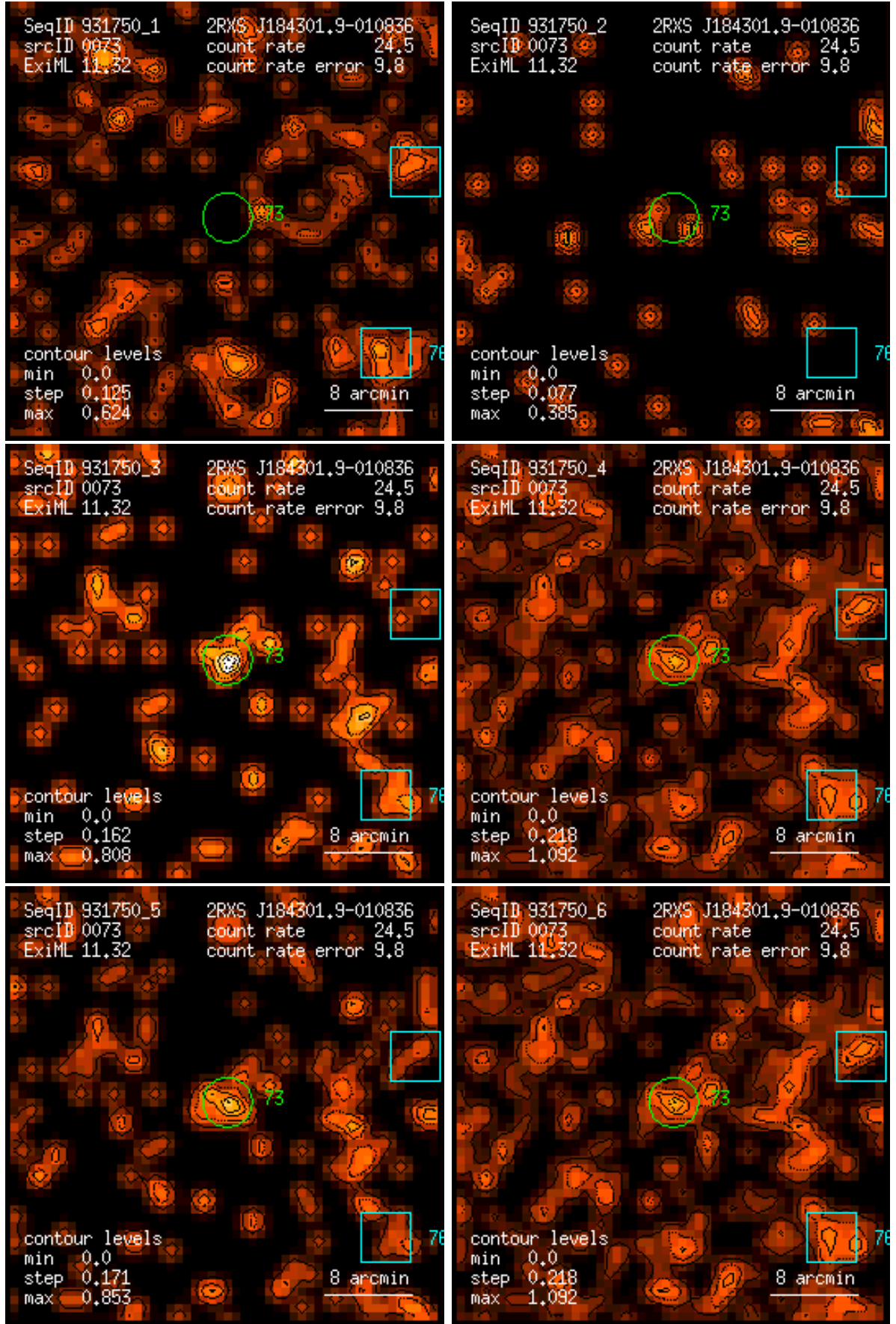
Figure 73: RASS 931750: detection 0073: band rate images, Gaussian filter: (1) PSPC channels 11 – 41, (2) 52 – 90, (3) 91 – 201, (4) 11 – 235, (5) 52 – 201, (6) 11 – 201. Broad band rates in counts/ks. Band rate contour levels in counts/ks/arcmin 2 .
