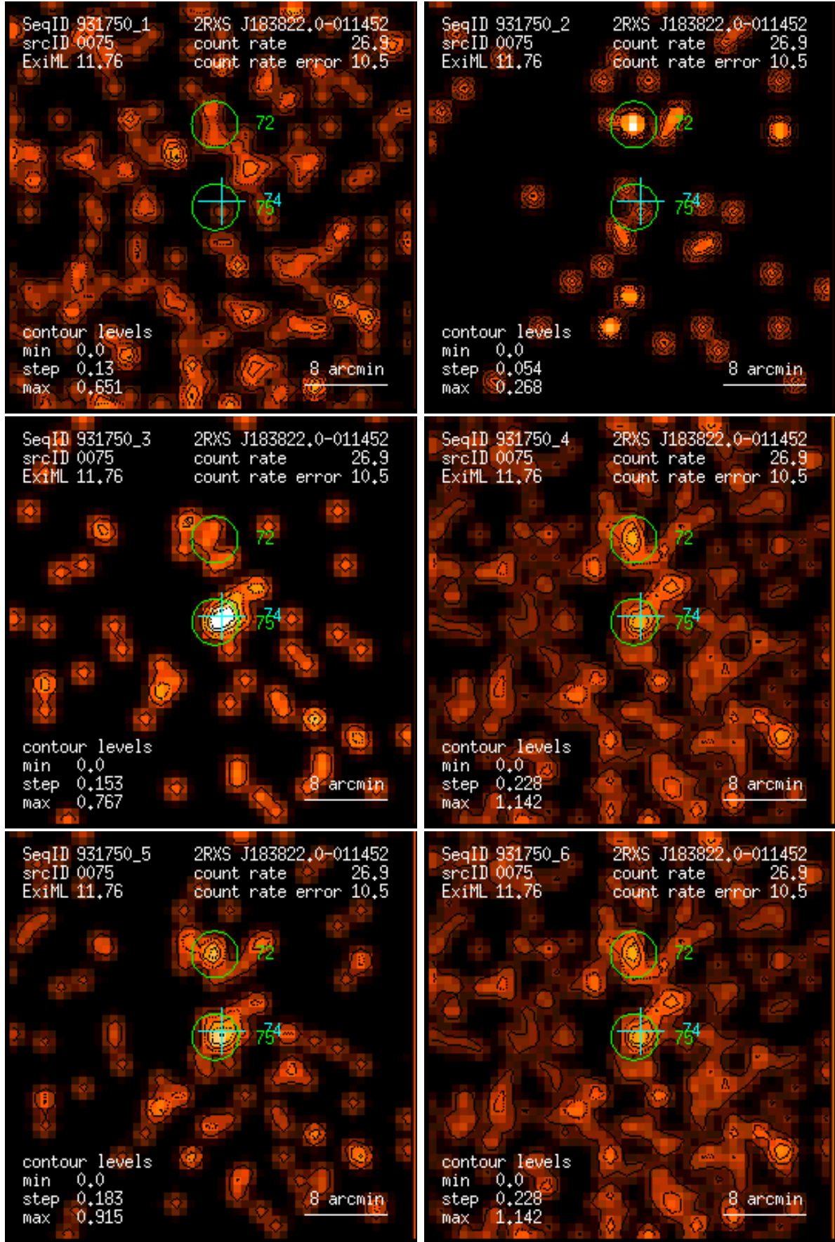
Figure 75: RASS 931750: detection 0075: band rate images, Gaussian filter: (1) PSPC channels 11 – 41, (2) 52 – 90, (3) 91 – 201, (4) 11 – 235, (5) 52 – 201, (6) 11 – 201. Broad band rates in counts/ks. Band rate contour levels in counts/ks/arcmin 2 .
