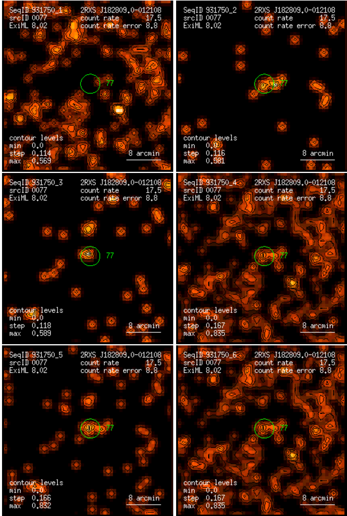
Figure 77: RASS 931750: detection 0077: band rate images, Gaussian filter: (1) PSPC channels 11 – 41, (2) 52 – 90, (3) 91 – 201, (4) 11 – 235, (5) 52 – 201, (6) 11 – 201. Broad band rates in counts/ks. Band rate contour levels in counts/ks/arcmin 2 .
