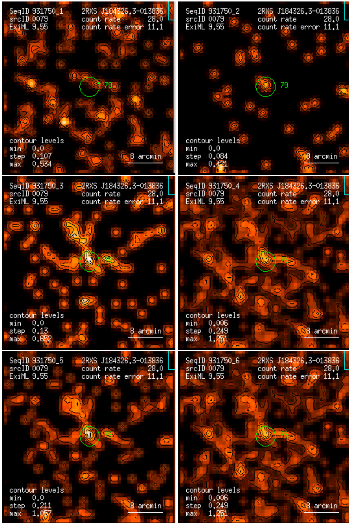
Figure 79: RASS 931750: detection 0079: band rate images, Gaussian filter: (1) PSPC channels 11 – 41, (2) 52 – 90, (3) 91 – 201, (4) 11 – 235, (5) 52 – 201, (6) 11 – 201. Broad band rates in counts/ks. Band rate contour levels in counts/ks/arcmin 2 .
