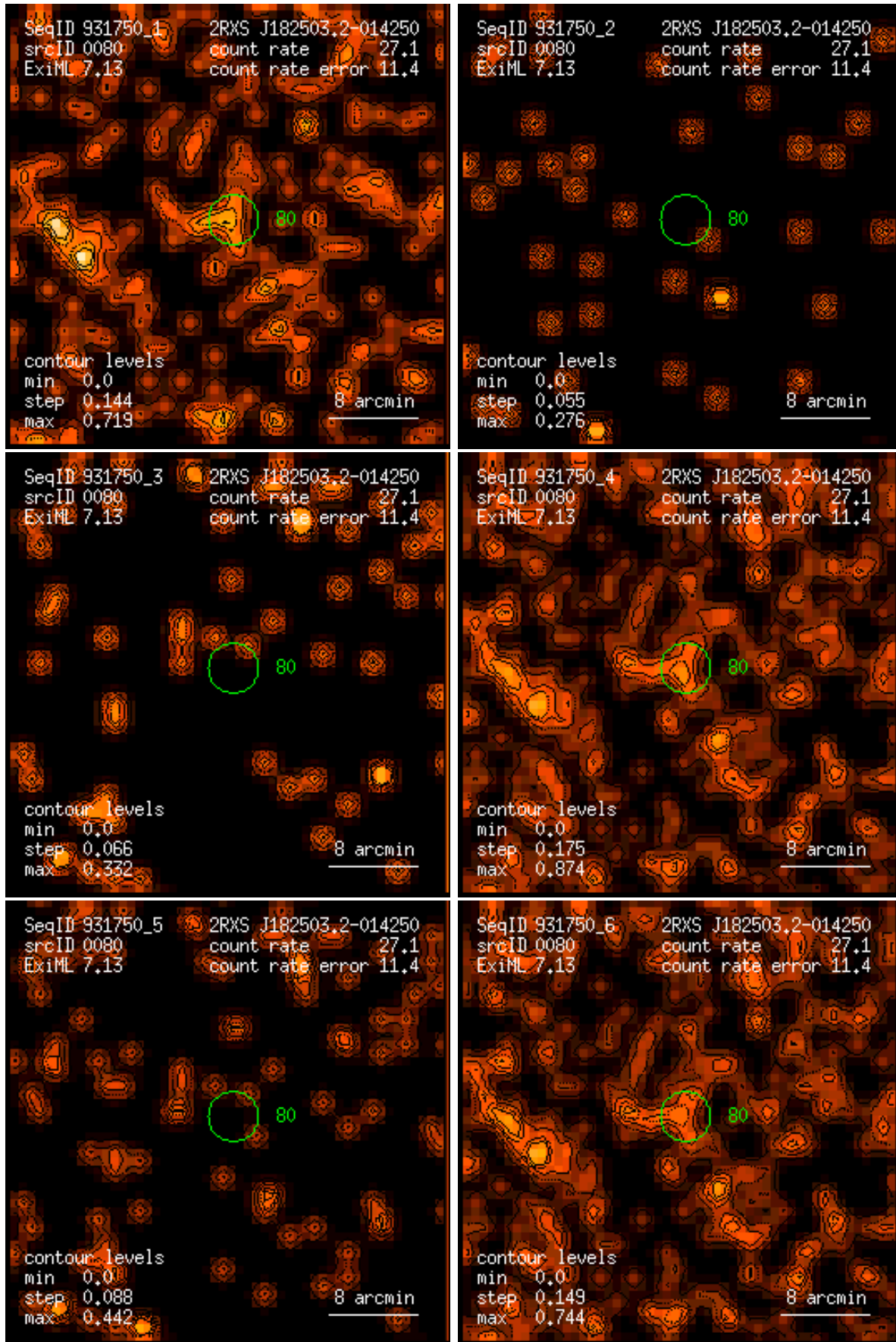
Figure 80: RASS 931750: detection 0080: band rate images, Gaussian filter: (1) PSPC channels 11 – 41, (2) 52 – 90, (3) 91 – 201, (4) 11 – 235, (5) 52 – 201, (6) 11 – 201. Broad band rates in counts/ks. Band rate contour levels in counts/ks/arcmin 2 .
