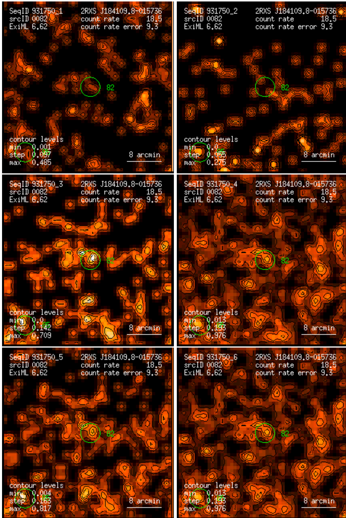
Figure 82: RASS 931750: detection 0082: band rate images, Gaussian filter: (1) PSPC channels 11 – 41, (2) 52 – 90, (3) 91 – 201, (4) 11 – 235, (5) 52 – 201, (6) 11 – 201. Broad band rates in counts/ks. Band rate contour levels in counts/ks/arcmin 2 .
